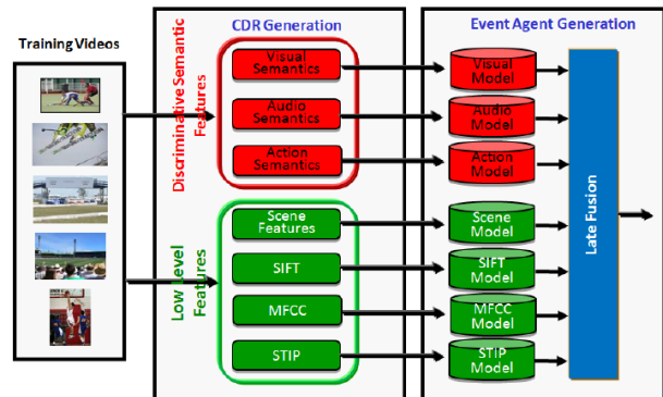
Figure 1: IBM/Columbia multimedia event detection system.
