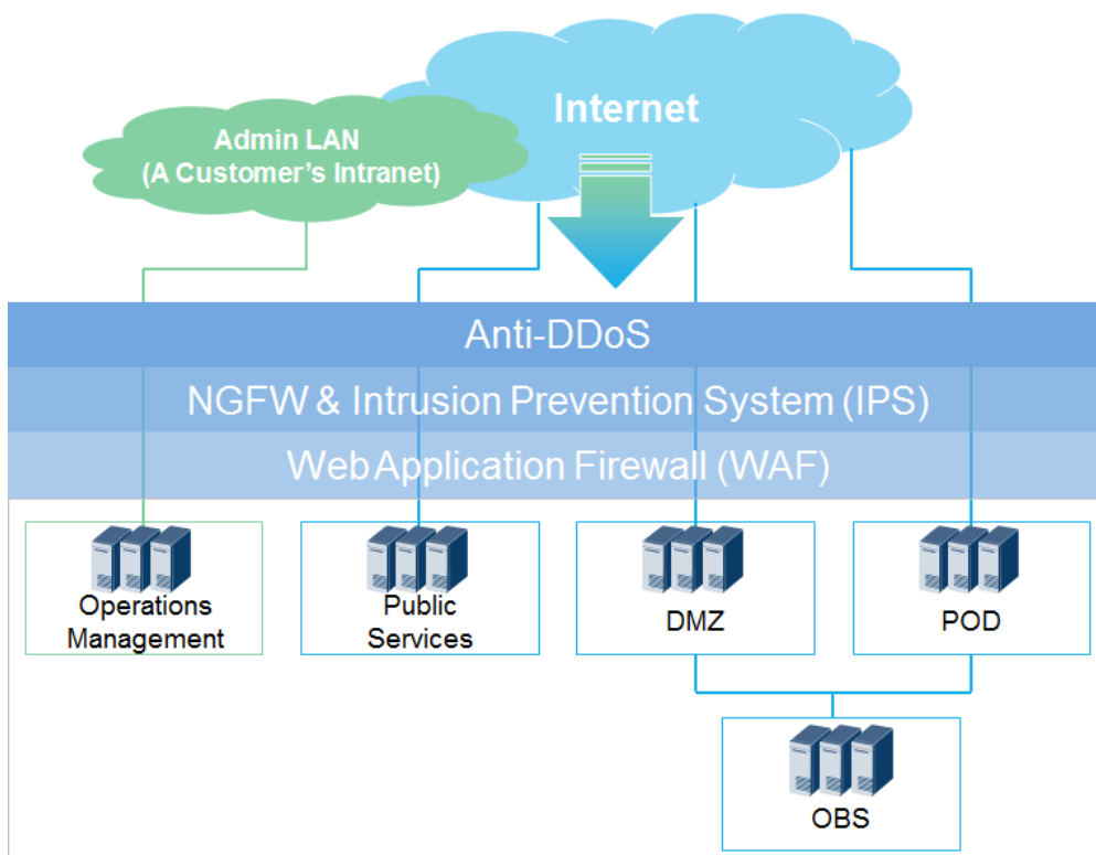
Figure 4-1 Huawei Cloud platform security zones and network border protection
