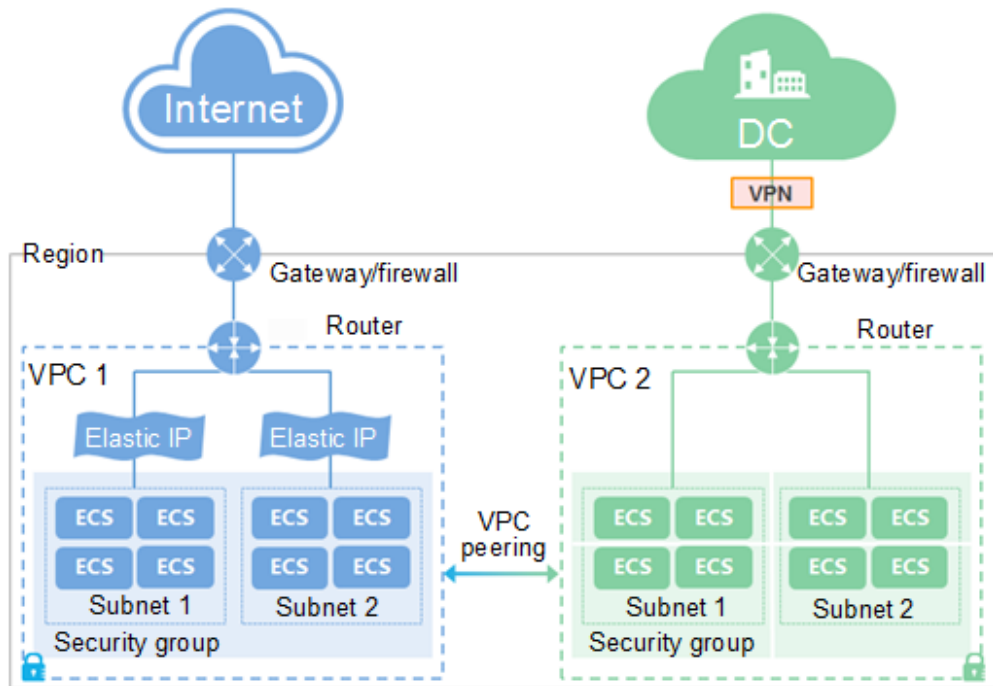
Figure 5-1 Huawei Cloud VPC architecture
