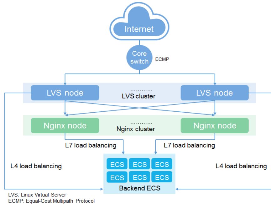
Figure 5-2 Huawei Cloud ELB networking diagram
