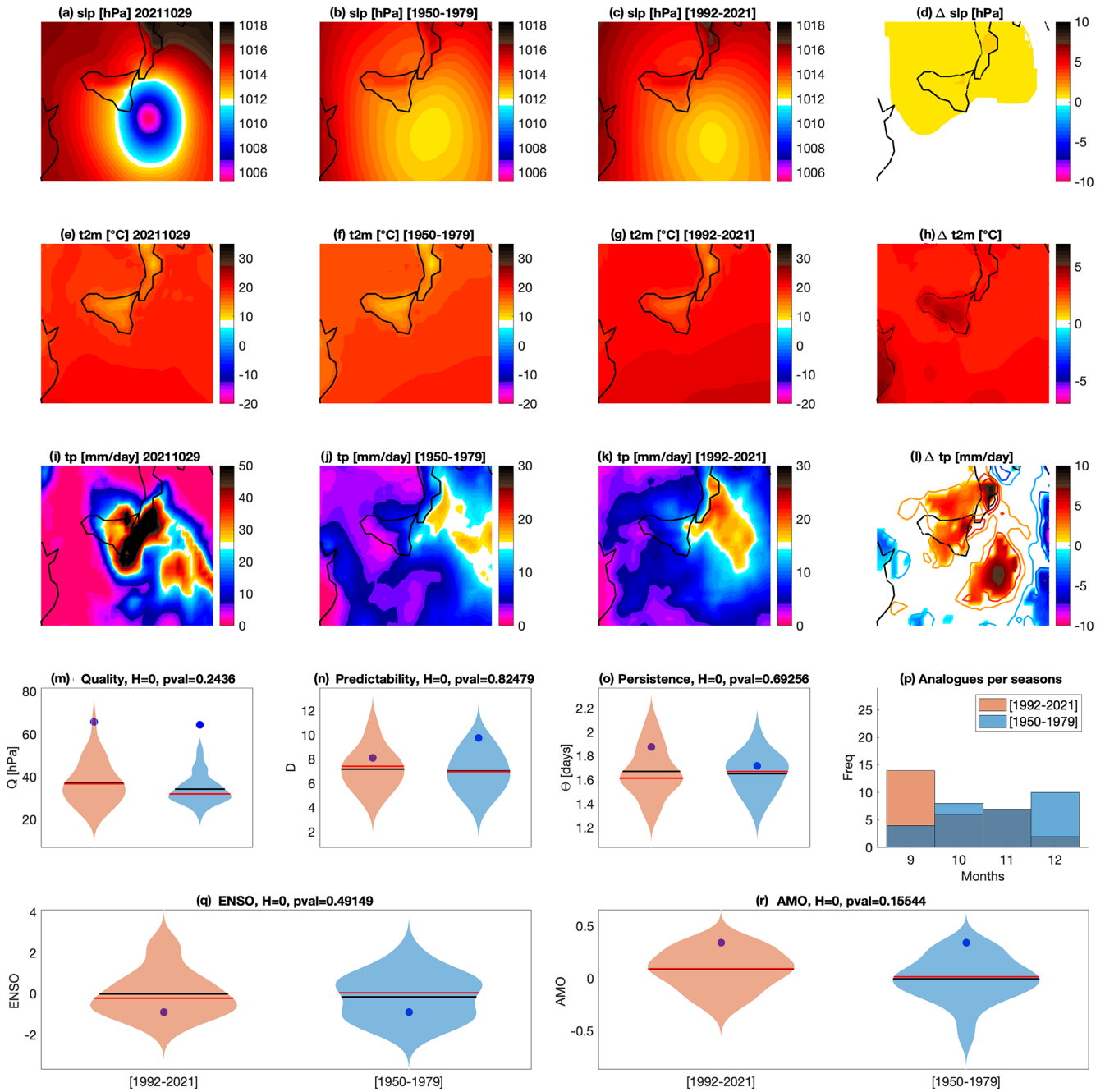
Figure 10. Attribution for the Medicane Apollo on 29 October 2021. Daily mean sea-level pressure slp (a), 2 m temperatures t2m (e) and total precipitation tp (i) on the day of the event. Average of the 33 sea-level pressure analogues found for the counterfactual [1950–1979] (b) and factual [1992–2021] (c) periods and corresponding 2 m temperatures (f, g) and daily precipitation rate (j, k). \Delta slp (d), \Delta t2m (h) and \Delta tp (l) between factual and counterfactual periods: colored–filled areas show significant anomalies with respect to the bootstrap procedure. Violin plots for counterfactual (blue) and factual (orange) periods for the analogue quality Q (m), the predictability index D (n), the persistence index \Theta (o) and the distribution of analogues in each month (p). Violin plots for counterfactual (blue) and factual (orange) periods for ENSO (q) and AMO (r). Values for the peak day of the extreme event are marked by a blue dot. Horizontal bars in panels (m)–(r) correspond to the mean (black) and median (red) of the distributions.
