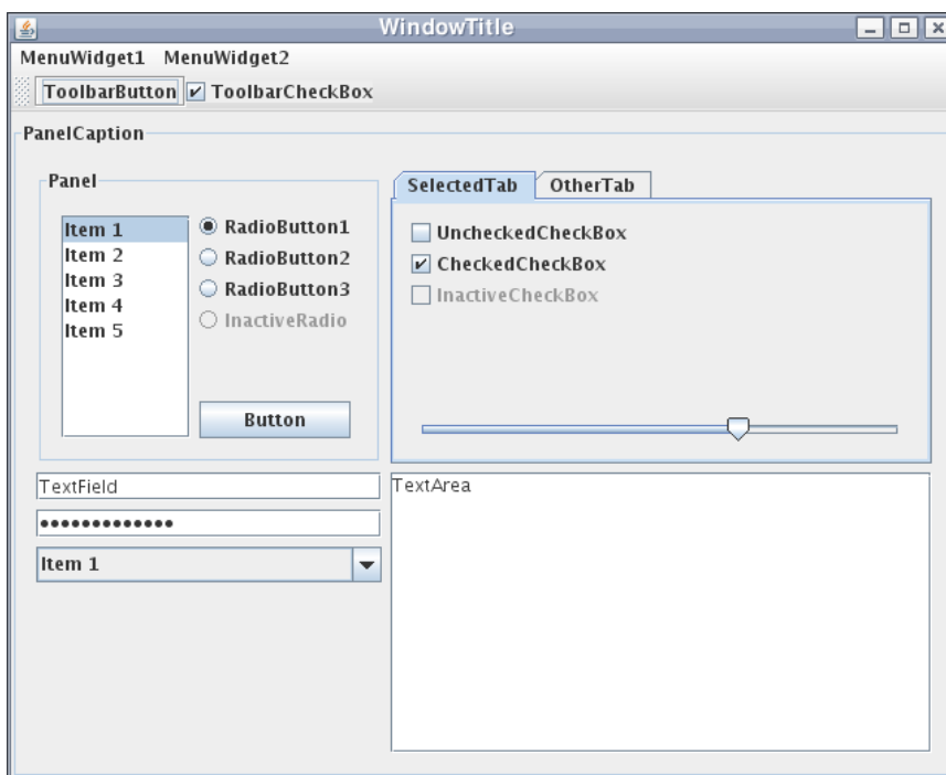
Figure 41 Swing does not rely on the underlying native user interface.
