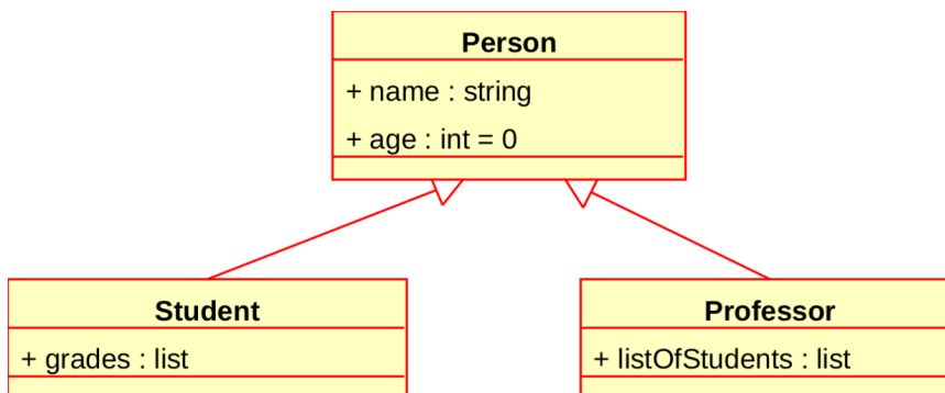
Figure 17 Object oriented programming can be represented with UML a diagrams.
