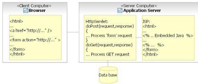
Figure 54 Figure 3: Jsp Execution
