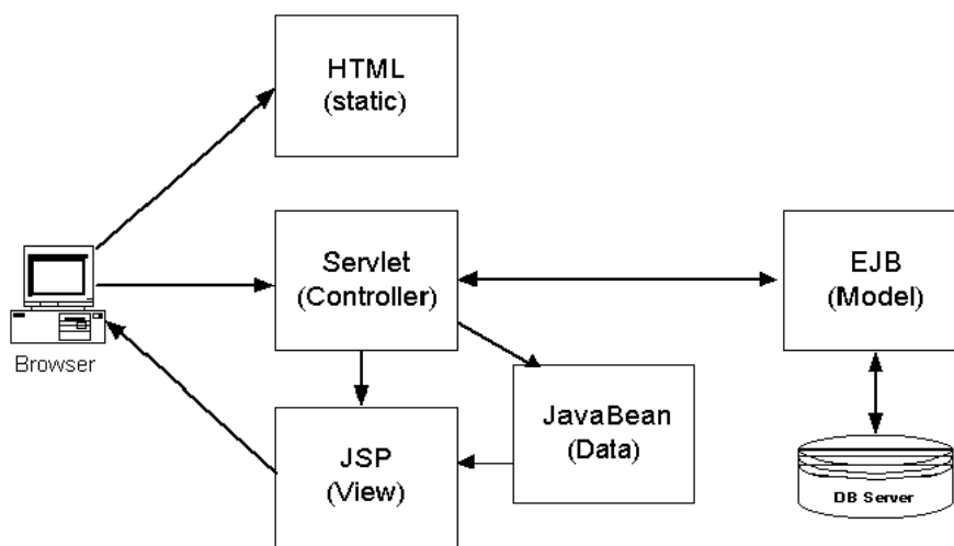
Figure 56 Figure 5: MVC Execution
