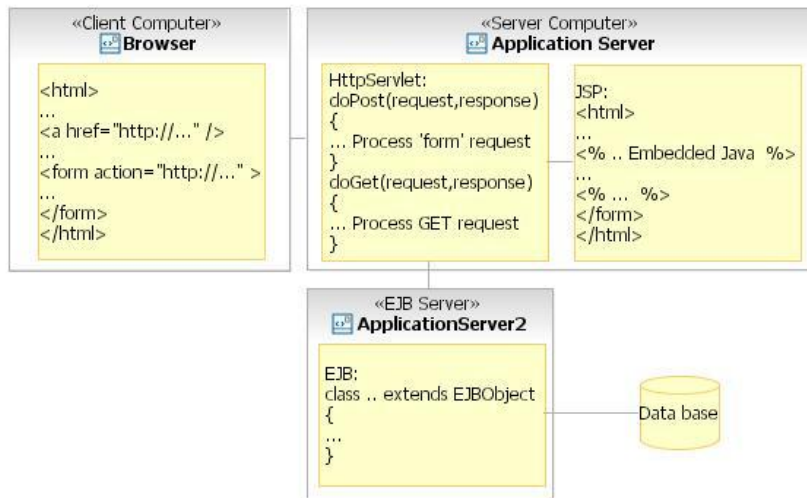
Figure 55 Figure 4: EJB Execution
