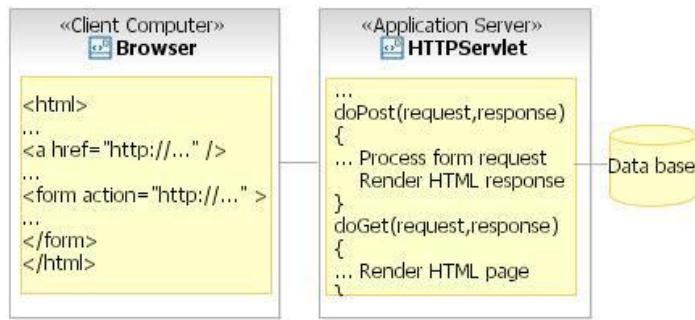
Figure 53 Figure 2: Servlet Execution
