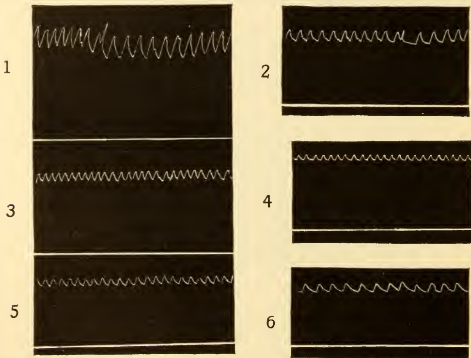
FIG. 13.—Showing changes in blood pressure and heart beat of Squalus due to transferrence from harbor water to fresh water from 11.06 A. M. to 3.56 P. M.
