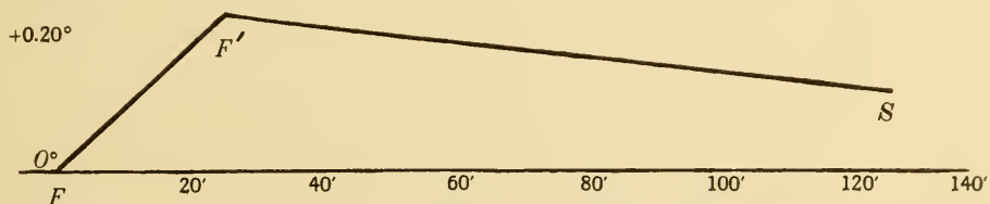
FIG. 5.—Changes in \Delta of blood of Mustelus due to immersion in fresh water followed by return to sea-water
