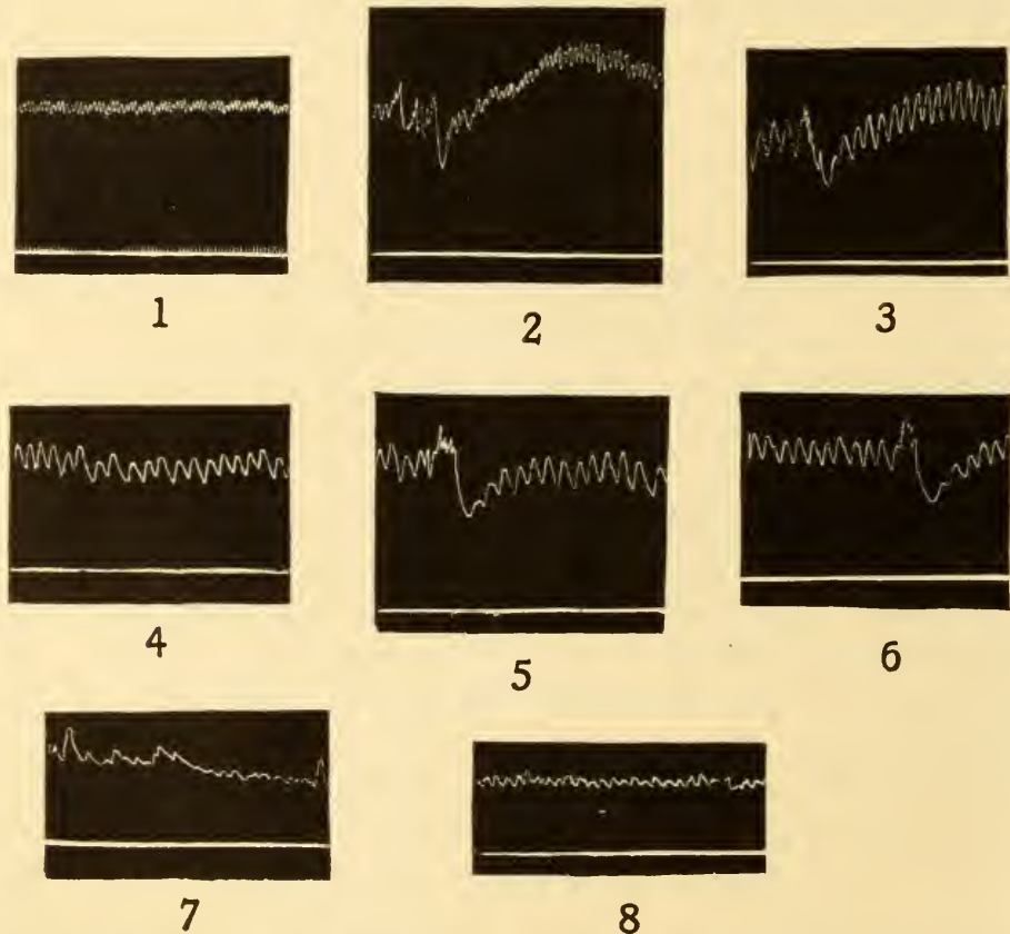
FIG. 10.—Showing changes in blood pressure of Mustelus canis due to immersion in fresh water
