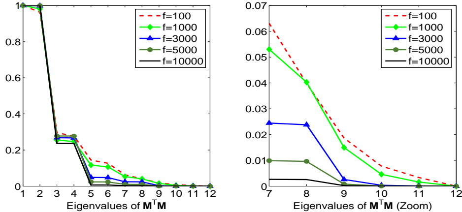
Fig. 3. Left: Singular values of M^T M for different focal lengths. Each curve averages 100 synthetic trials. Right: Zooming in on the smallest eigenvalues. For small focal lengths, the camera is perspective and only one eigenvalue is zero, which reflects the scale ambiguity. As the focal length increases and the camera becomes orthographic, all four smallest eigenvalues approach zero.
