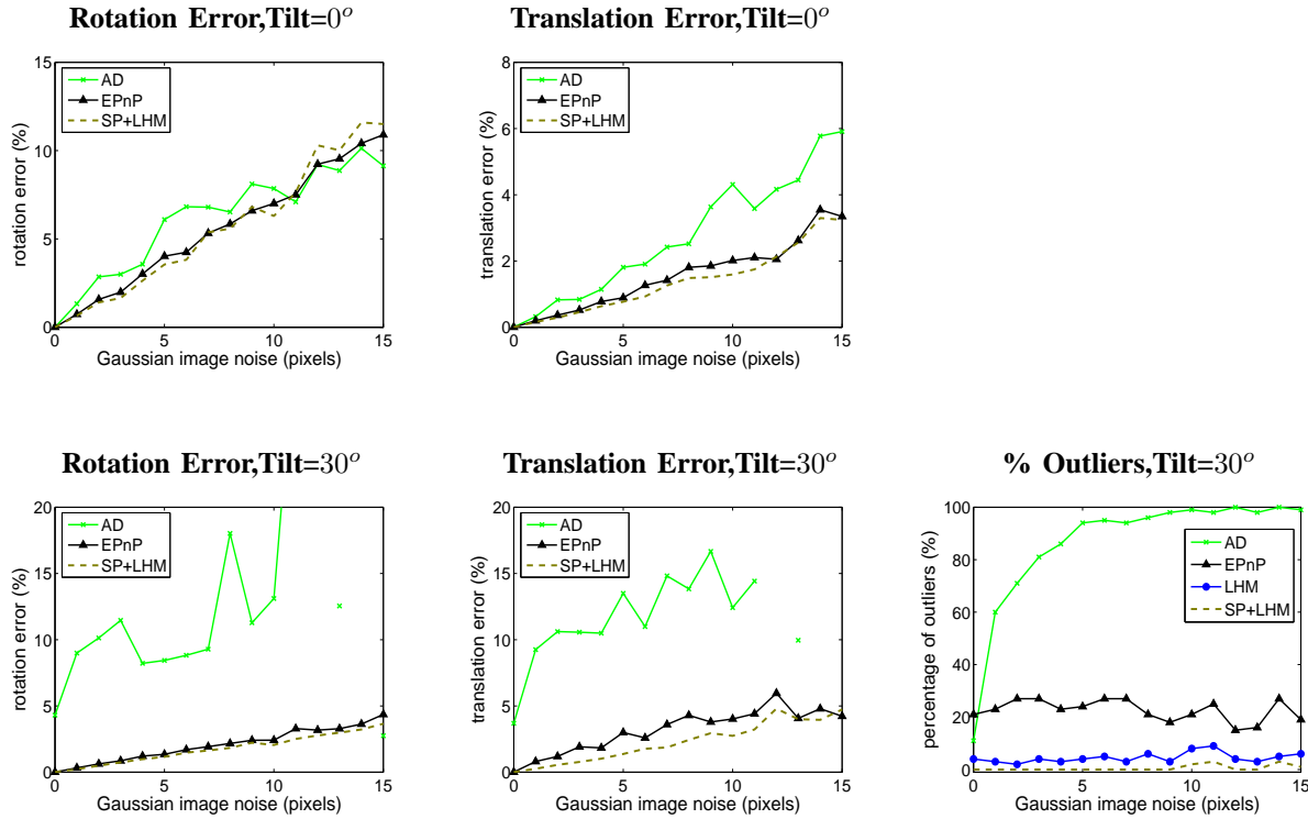
Fig. 7. Planar case. Errors as a function of the image noise when using n = 6 reference points. For \text{Tilt}=0^\circ , there are no pose ambiguities and the results represent the mean over all the experiments. For \text{Tilt}=30^\circ , the errors are only averaged among the solutions not affected by the pose ambiguity. The right-most figure represents the number of solutions considered as outliers, which are defined as those for which the average error in the estimated 3D position of the reference points is larger than a threshold.
