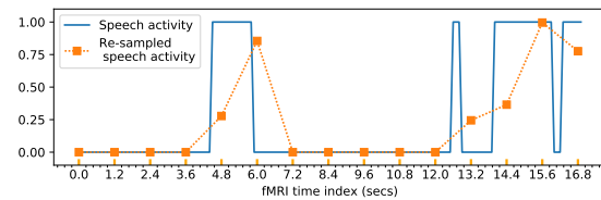
Figure 2: Example of resampling speech features (the speech activity).
