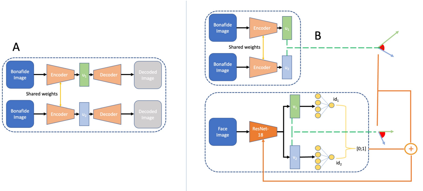
Fig. 1. Overall scheme of the architecture. Part A represents the training of the autoencoder, whereas part B represents the training of the classification system. The orange line represents the backpropagation, the green one represents the calculation of the angle between vectors and the yellow represents the fusion of the two scores. Best viewed in color.
