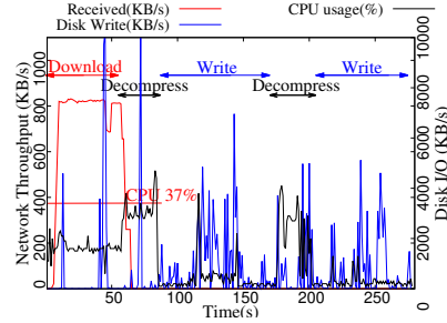
(b) Ubuntu image with a 1 Mbps network cap.
