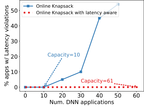
Fig. 16. Latency violations under different co-location methods
