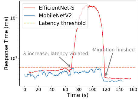
Fig. 20. Hotspot mitigation with token bucket.
