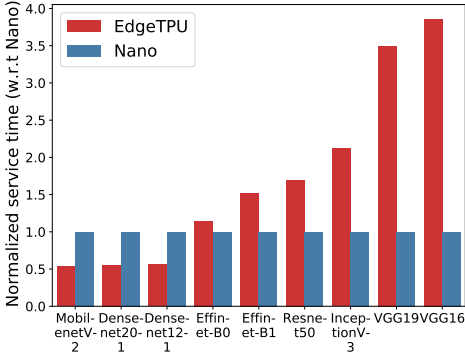
Fig. 15. Normalized service time for various DNN models.
