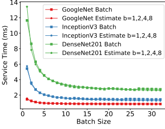
Fig. 10. GPU response times for batched request execution.
