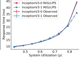
Fig. 11. Response time under MPS for two DNNs with c=1.65 .
