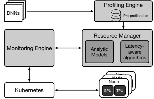
Fig. 14. Ibis implementation overview
