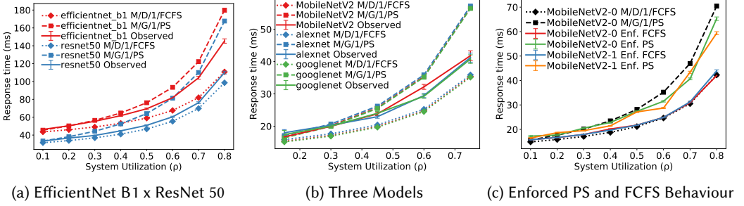
Fig. 9. GPU behaviour with multiple applications per node.
