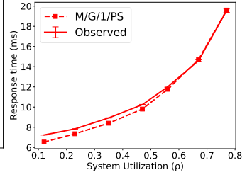
Fig. 12. CPU response times at different utilization levels.
