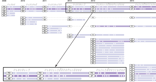
Figure 4. Visualizing the ego-network of P. Dragicevic (PD) using an unpacked view, compared to the compact view in Figure 1. The line colors indicate the betweenness centrality of actors at different time steps using a white-purple color scheme. By tracing the color of the actor line of JF, a valley of the betweenness centrality metric is observed in 2013 (magnified here).
