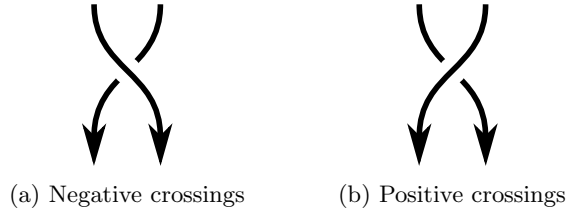
Fig. 8. Sign convention for torsions, permutations and crossings.
