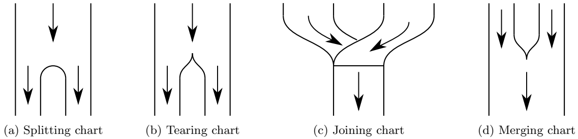
Fig. 4. The different charts that can be used to draw a template.
