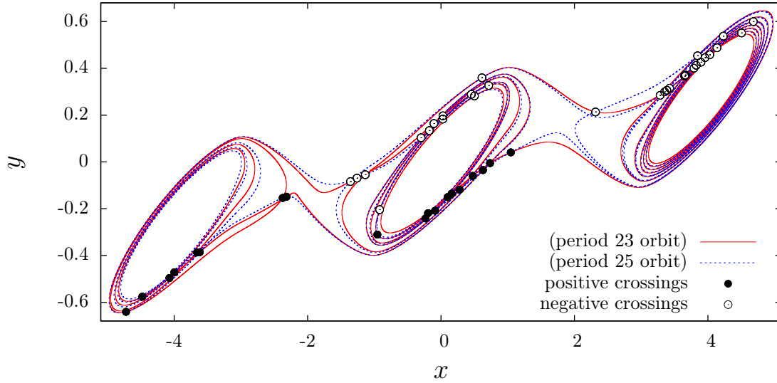
Fig. 16. Two unstable periodic orbits extracted from the chaotic multispiral attractor solution to equations (16). Their orbital sequences are (\overline{7} \ 0 \ \overline{0} \ 0 \ \overline{1} \ 3 \ 4 \ 4 \ 4 \ 4 \ 4 \ 4 \ 7 \ \overline{0} \ 0 \ \overline{0} \ 0 \ \overline{0} \ 0 \ \overline{3} \ \overline{4} \ \overline{4} \ \overline{5}) and (\overline{7} \ 0 \ \overline{0} \ 0 \ \overline{0} \ 0 \ \overline{1} \ 3 \ 4 \ 4 \ 4 \ 4 \ 4 \ 5 \ 4 \ 4 \ 7 \ \overline{0} \ 0 \ \overline{0} \ 0 \ \overline{3} \ \overline{4} \ \overline{4} \ \overline{4}) . The linking number between these two orbits is -6 . Parameter values are those of Fig. 12.
