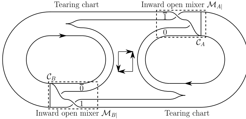
Fig. 11. Template that describes the Lorenz attractor shown in Fig. 9.
