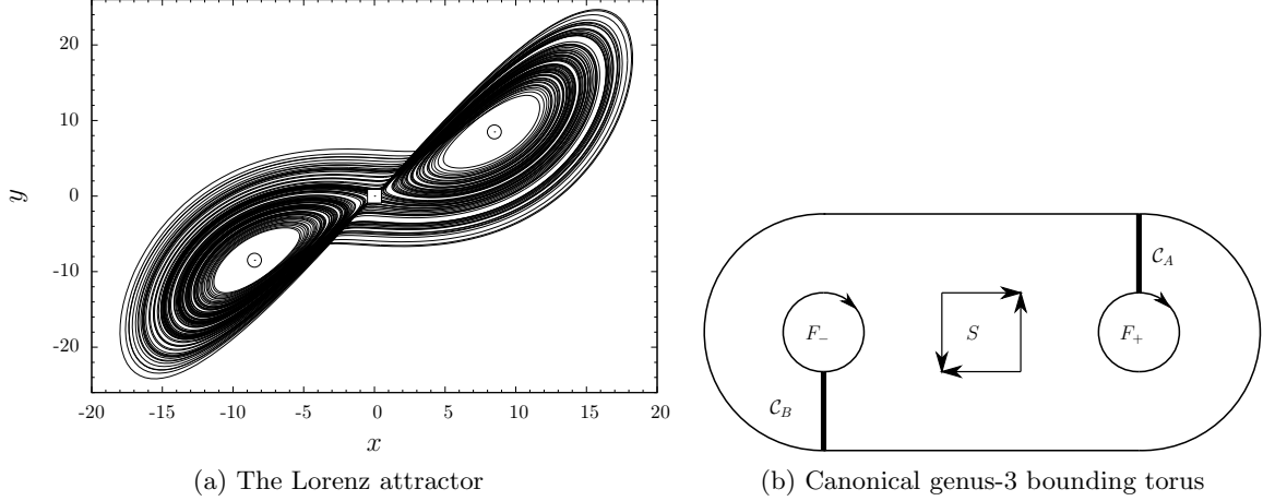
Fig. 9. Chaotic attractor solution to the Lorenz equations (8) and its singular points ( \odot for saddle-focus points and \boxtimes for the saddle point). The canonical form of the corresponding bounding torus is also shown with the two components \mathcal{C}_A and \mathcal{C}_B of the Poincaré section. Parameter values R = 28 , \beta = \frac{8}{3} and \sigma = 10 .
