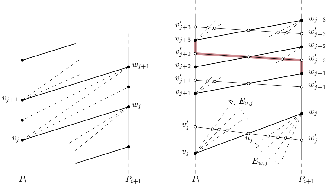
Figure 4 Left: Several inter-path-edges between P_i and P_{i+1} . Only the solid ones are non-transitive in G'[\mathcal{P}] . Right: The comparability between w'_j and v'_j was achieved by adding a w'_j - v'_j -path. To preserve that G' is a planar st -graph, all intersected edges are subdivided at the intersections. Further the comparability w_{j+1} \prec_{G'} v_{j+3} is highlighted. Note that the dashed edges may have only one endpoint in P_i or P_{i+1} .
