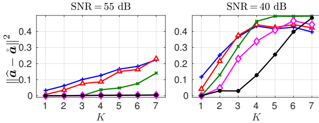
Fig. 2. Error on estimated abundances for FCLS (+), GE ( \Delta ), \ell_0 ( \circ ), SA+GE ( \diamond ), and backward [12] ( \times ).
