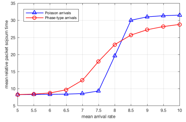
Fig. 4: Example II: mean relative packet sojourn time as a function of load for non-Poisson and Poisson arrival processes.
