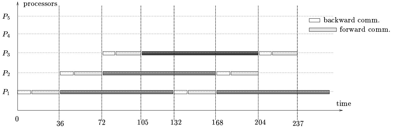
Figure 13: Pattern when communications are required both before and after each task
