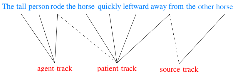
Figure 4: The order of cross products required to encode the meaning of a sentence is not arbitrary and is shown here by the arrows connecting each word to each tracker, shown in red. The number of tracks is determined by parsing the sentence. The lattices for words or lexicalized phrases such as away from are cross producted with the tracks that those words refer to. The dashed line indicate that the order of the cross products is essential for words which have more than one role, in other words rode is not symmetric.
