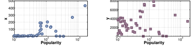
(a) Number of replicas \mathbf{x} . (b) Deadlines \mathbf{y} (in s ). Fig. 3: Example of an allocation for QAC (semilog scale).
