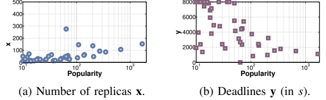
Fig. 4: Example of an allocation for QAC-SC (semilog scale).
