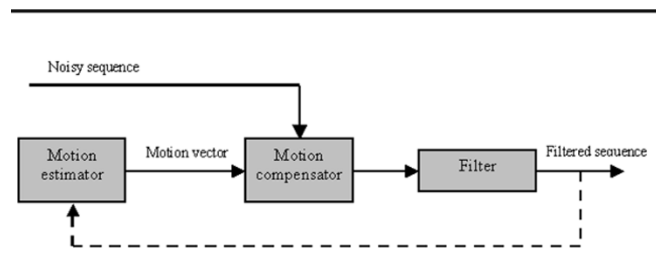
Fig. 1. Motion-compensated filtering scheme consists of three parts: first, the motion is estimated; second, the observed temporal signal is compensated for motion; third, it is filtered.
