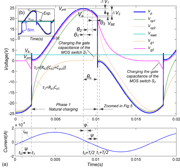
Fig. 4. (a) Simulated waveforms of the SP-OSECE circuit; (b) Comparison of experimental and simulated waveforms. Solid lines: experimental; Dashed lines: simulated.
