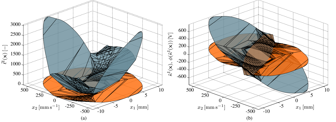
Fig. 2. Illustration of the inverse parametric optimization ( N = 2 ) based EMPC implementation (acc. Section II-C1) for the experimental vibration system. (a) A convex lifting \bar{\ell}^I(\mathbf{x}) and the associated state-space partition \bar{\mathcal{R}}^I (for illustration only). (b) The recovered PWA control law \bar{\kappa}^I(\mathbf{x}) in blue, and the result of clipping \phi(\bar{\kappa}^I(\mathbf{x})) at \bar{\kappa} = 100 and \underline{\kappa} = -100 in orange color (illustration only, cf. Fig. 1); \bar{R}^I = 1160 .
