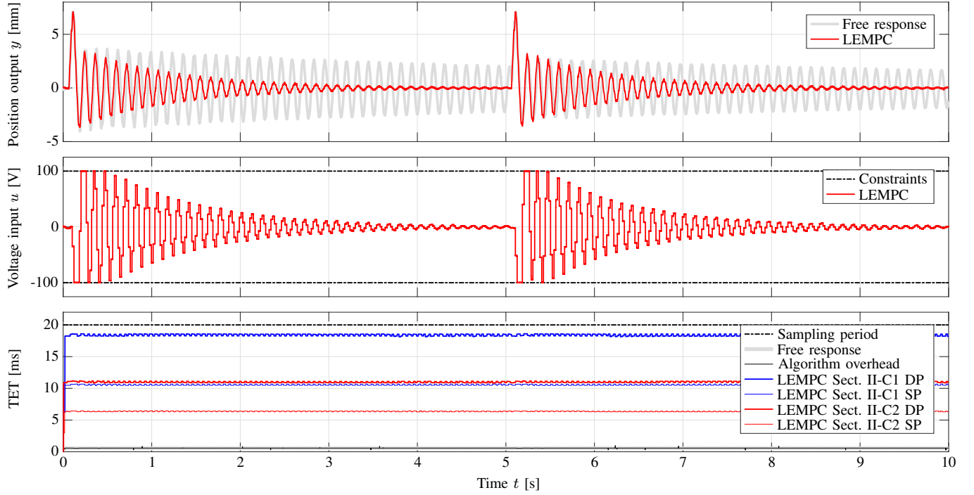
Fig. 8. Typical output, input and timing profiles for the laboratory release tests (two cycles) using the active cantilever beam and the F051x MCU; DP (SP) denotes Double(Single)-Precision floating-point format.
