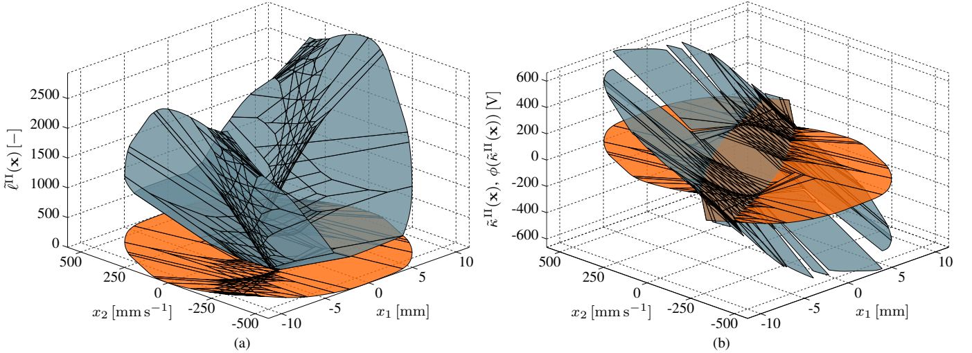
Fig. 3. Illustration of the convex lifting based EMPC implementation (acc. Section II-C2) for the experimental vibration system. (a) A convex lifting \bar{\ell}^{II}(\mathbf{x}) and the associated state-space partition \bar{\mathcal{R}}^{II} (for illustration only). (b) The associated PWA control law \bar{\kappa}^{II}(\mathbf{x}) in blue, and the result of clipping \phi(\bar{\kappa}^{II}(\mathbf{x})) at \bar{\kappa} = 100 and \underline{\kappa} = -100 in orange color (illustration only, cf. Fig. 1); \bar{R}^{II} = |\mathcal{I}_{\text{uns}}| = 679 .
