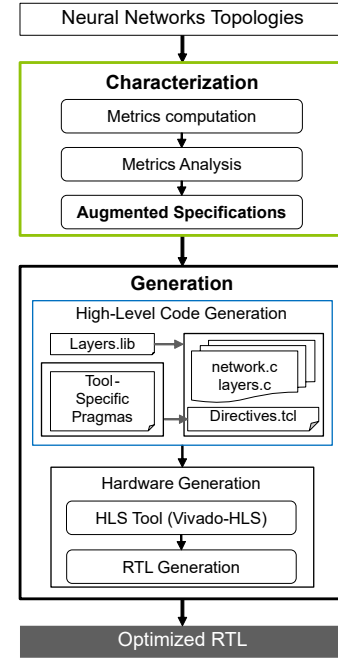
Fig. 2. Overview of the proposed exploration and accelerator generation framework flow.
