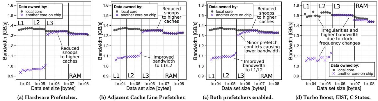
Figure 9: The effect on the bandwidth of FAA (accessing cache lines in the Modified state) coming from prefetchers and various power efficiency and acceleration mechanisms (Turbo Boost, EIST, C States) deployed in Intel Haswell.
