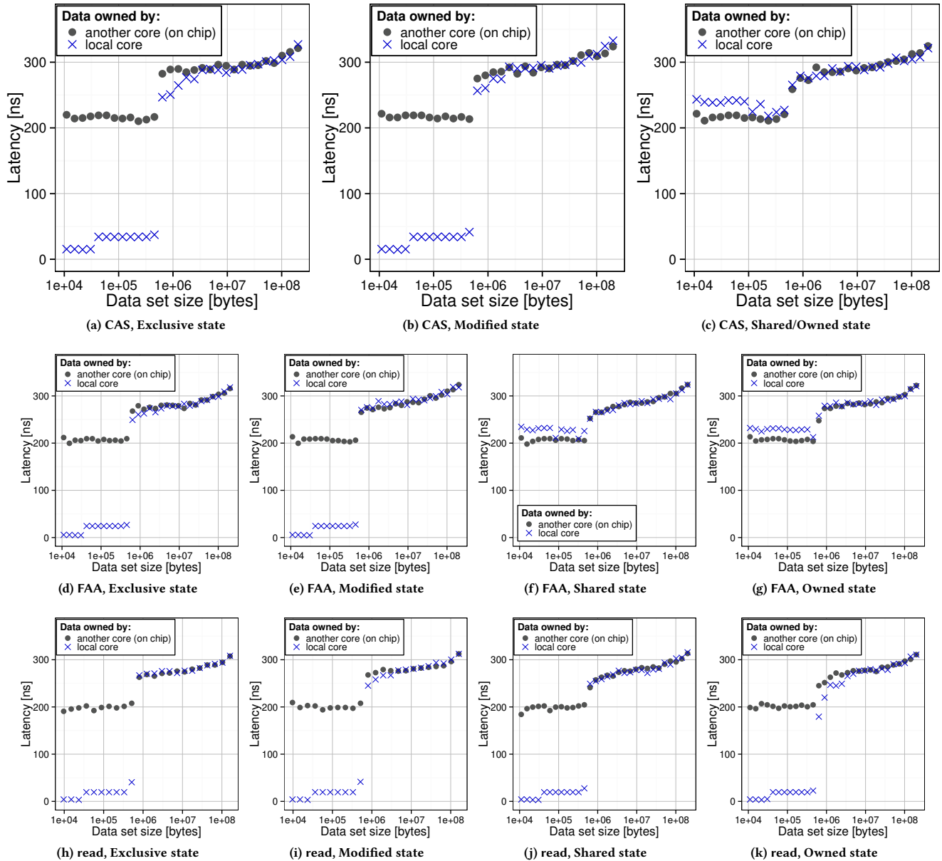
Figure 11: The comparison of the latency of CAS, FAA, and read on Xeon Phi. The requesting core accesses its own cache lines (local) and cache lines of a different core from the same chip (on chip).
