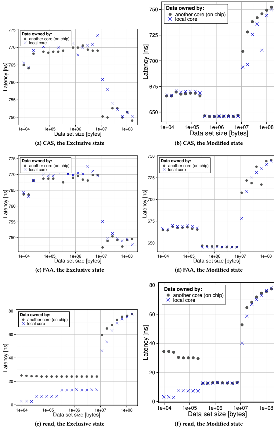
Figure 14: The comparison of the latency of unaligned CAS, FAA, and read on Haswell. The requesting core accesses its own cache lines (local) and cache lines of a different core from the same chip (on chip)
