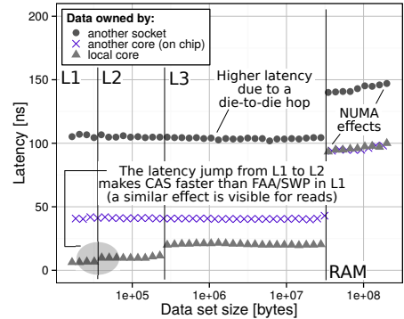
Figure 3: The analysis of the CAS latency (Exclusive state) on Ivy Bridge and the comparison to FAA/SWP. The requesting core accesses its own cache lines (local), cache lines of a different core from the same chip (on chip), and cache lines of a core from a different socket (another socket).
