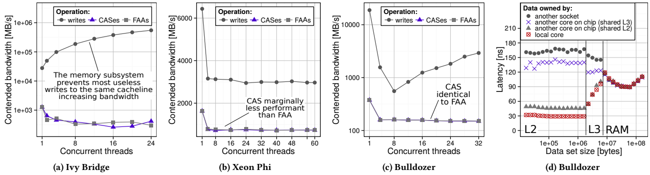
Figure 8: Figures 8a-8c illustrate the comparison of the contended bandwidth of CAS/FAA/writes on Ivy Bridge, Bulldozer, and Xeon Phi. Figure 8d shows the latency of CAS that fetches two operands from the memory subsystem on Bulldozer (Exclusive state).
