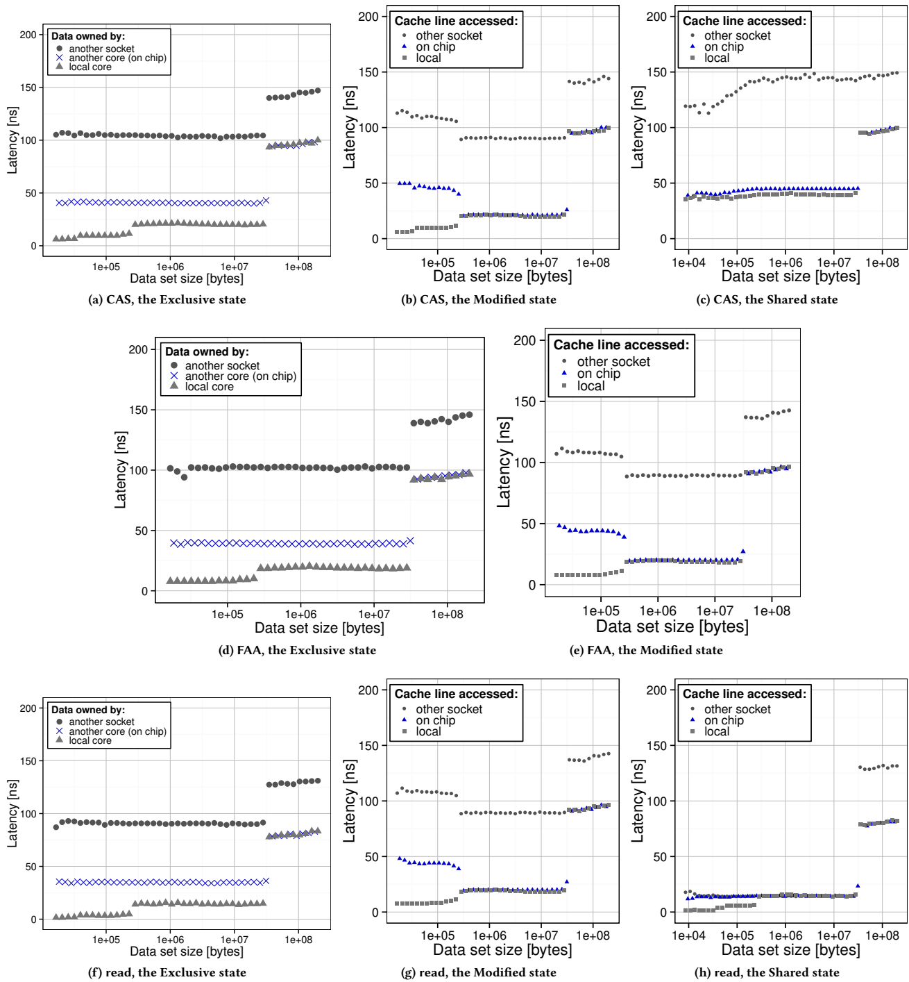
Figure 12: The comparison of the latency of CAS, FAA, and read on Ivy Bridge. The requesting core accesses its own cache lines (local), cache lines of a different core from the same chip (on chip), and cache lines of a different core from a different socket (other socket).
