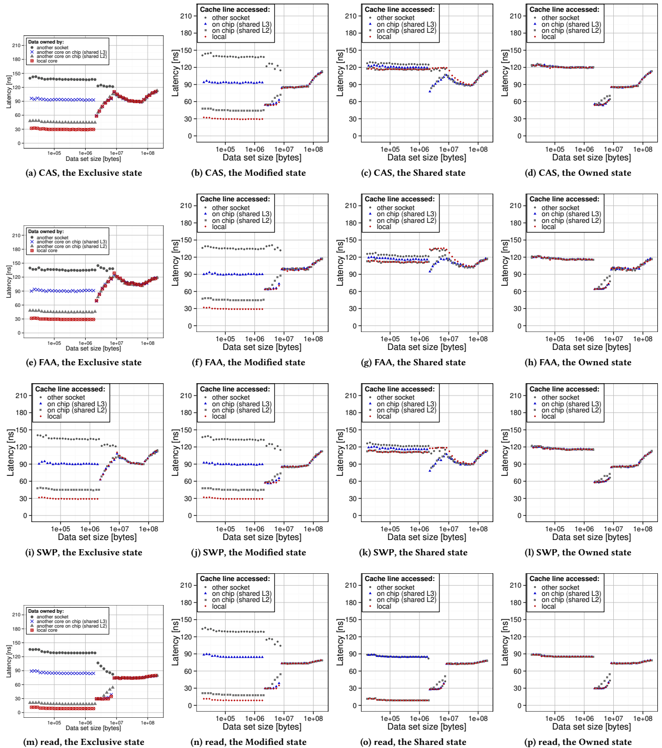
Figure 13: The comparison of the latency of CAS, FAA, SWP, and read on Bulldozer. The requesting core accesses its own cache lines (local), cache lines of different cores that share L2 and L3 with the requesting core (on chip, shared L2 and L3, respectively), and cache lines of a different core from a different socket (other socket).
