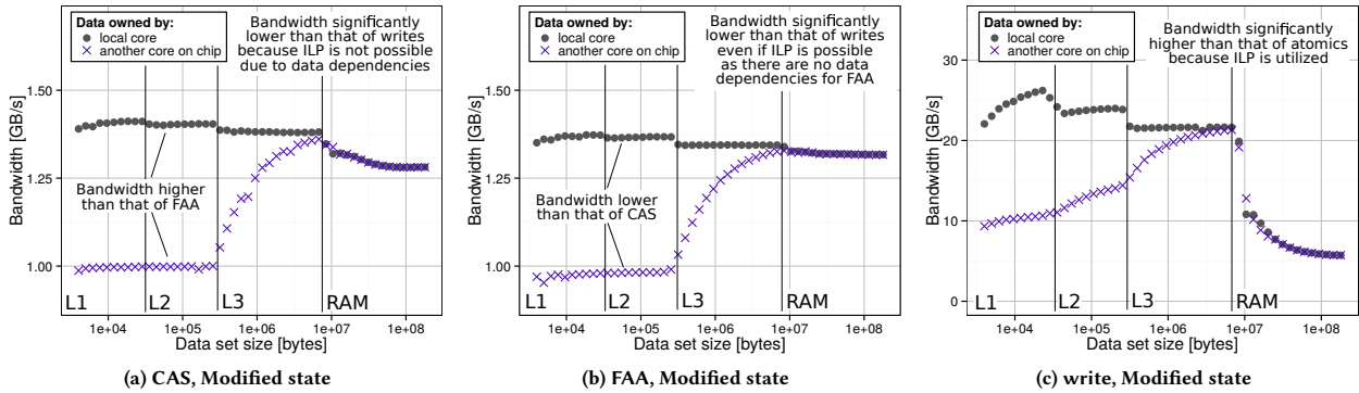
Figure 5: The comparison of the bandwidth of CAS, FAA, and writes on Haswell. The requesting core accesses its own cache lines (local) and cache lines of a different core from the same chip (on chip).
