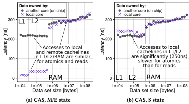
Figure 6: The comparison of the latency of CAS on Xeon Phi. The requesting core accesses its own cache lines (local) and cache lines of a different core from the same chip (on chip).
