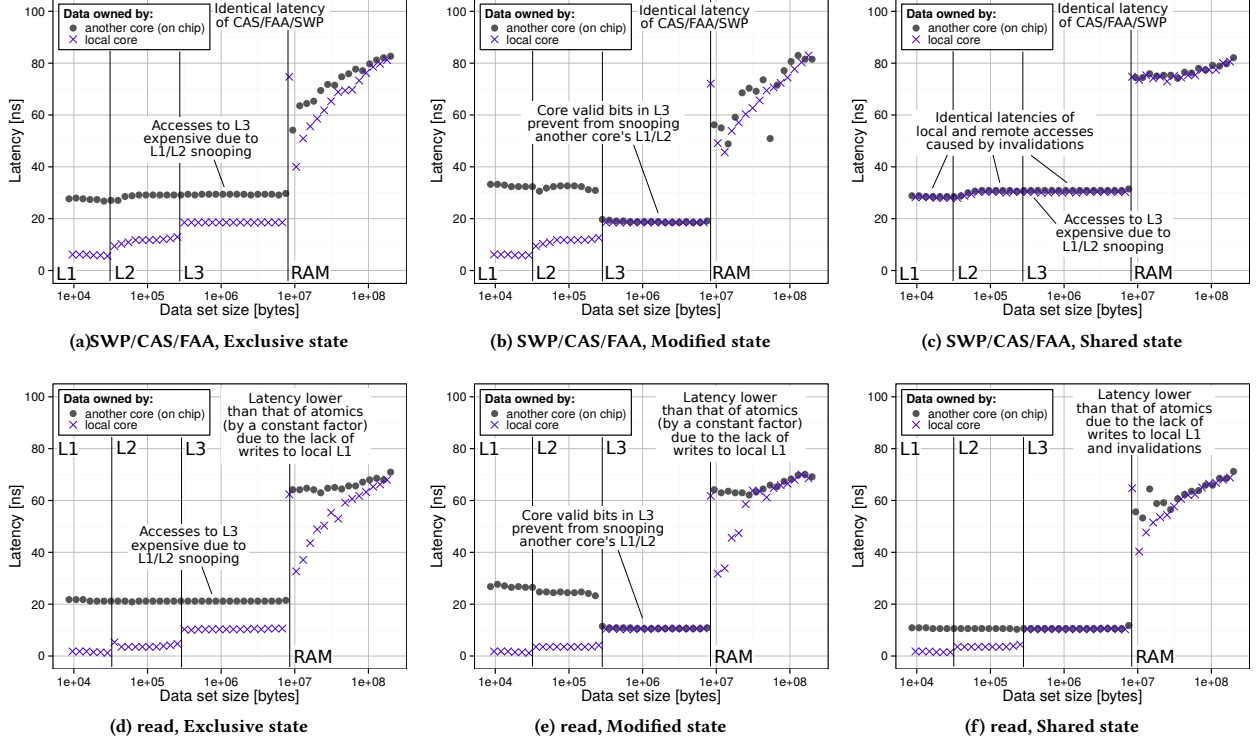
Figure 2: The comparison of the latency of CAS, FAA, SWP, and read on Haswell. The requesting core accesses its own cache lines (local) and cache lines of a different core from the same chip (on chip).
