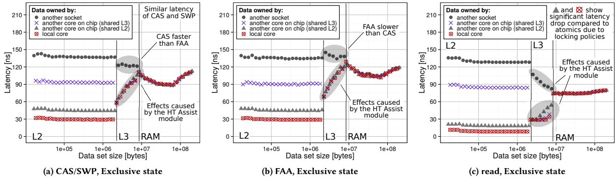
Figure 4: The latency comparison of CAS/FAA/SWP/read on Bulldozer. The requesting core accesses its own cache lines (local), cache lines of different cores that share L2 and L3 with the requesting core (on chip, shared L2 and L3, respectively), and cache lines of a core from a different socket (other socket).
