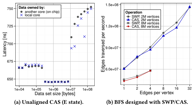
Figure 10: The analysis of unaligned atomics and BFS.
