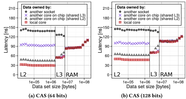
Figure 7: The comparison of the latency of CAS using operands of 64 and 128 bits in size (AMD Bulldozer, the M state).
