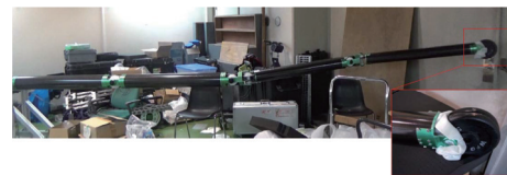
Fig. 18. 5.7 m model lifting 10 kg weight.
