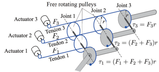
Fig. 3. Basic principle of the coupled tendon-driven mechanism.
