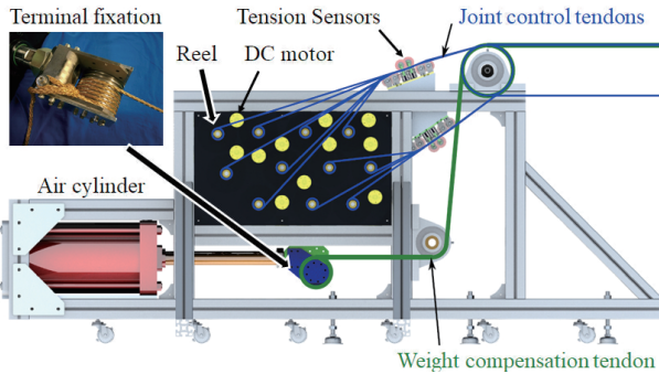
Fig. 9. Base structure: arrangement of the actuators and the tendon pathways.
