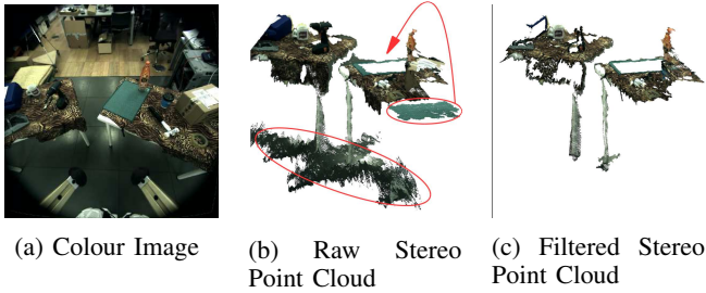
Fig. 4: The raw disparity images are filtered to remove unreliable data. (a) is the original colour image. (b) is the corresponding raw stereo point cloud - red circles highlight erroneous depth from areas of low texture, such as the floor and a green sheet reconstructed apart from its actual location (indicated with an arrow). (c) is the result of our filtering procedure.
