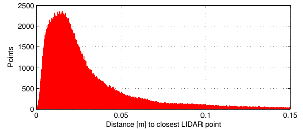
Fig. 10: Distribution of stereo points error.
