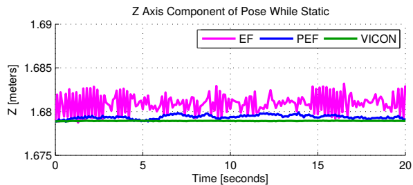
Fig. 7: Z-component of the robot's pose for a sequence in Log1 when it is stationary: fusion of kinematic-inertial within visual tracking (PEF) results in more stable pose than using only vision (EF).
