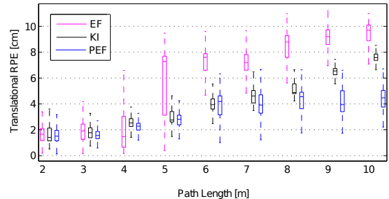
Fig. 6: Translational RPE (cm) for increasing path lengths (m) for Log1, showing PEF achieving the smallest drift rate.
