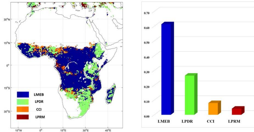
Figure 1. Left: the distribution of the model which produced the highest temporal correlation; right: the histogram of the percentage for each model with the highest temporal correlation.
