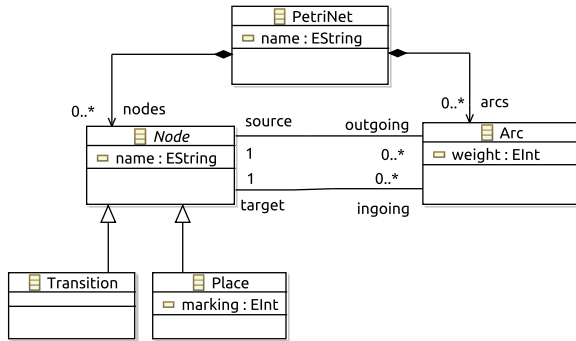
Figure 2. A metamodel for Petri nets, slightly modified from [13].
