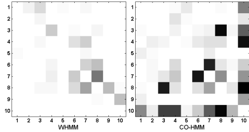
Figure 6. Occurring phase transitions, on-line, for WHMMs and CO-HMMs. White color means absence of transition.
