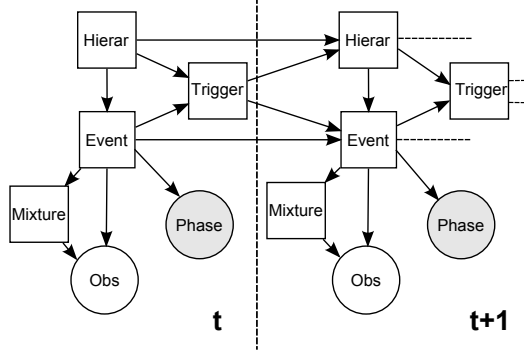
Figure 3. Dynamic Bayesian Network (DBN) representation of the WHMMs: two-levels hierarchy with a phase variable.
