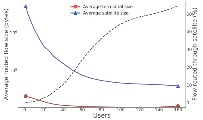
Fig. 4: Average flow size on each path with the MinFCT scheme.
