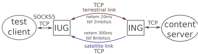
Fig. 2: Experimental testbed architecture.
