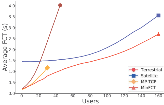
Fig. 3: Comparison of average Flow Completion Time with MinFCT, MP-TCP, TCP over the terrestrial path only and TCP over the satellite path only.
