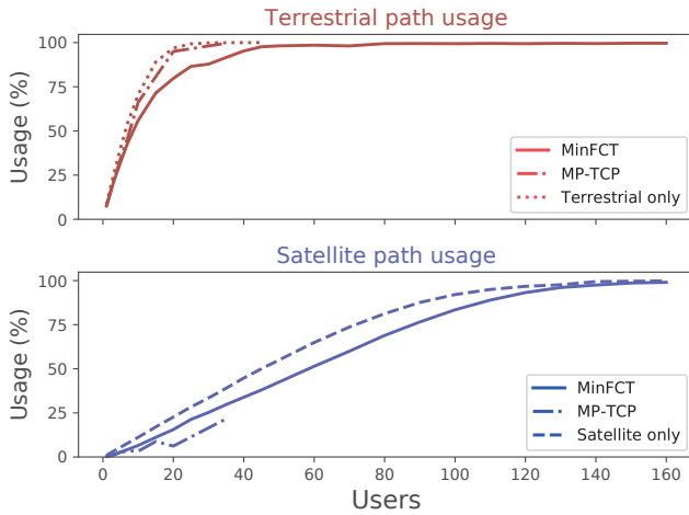
Fig. 5: Occupancy rate for terrestrial and satellite path, considering routing through the terrestrial path only, satellite path only, with MP-TCP or with the MinFCT algorithm.
