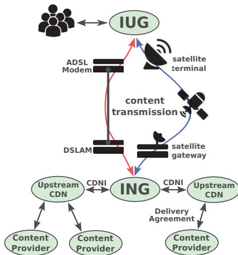
Fig. 1: Hybrid architecture
