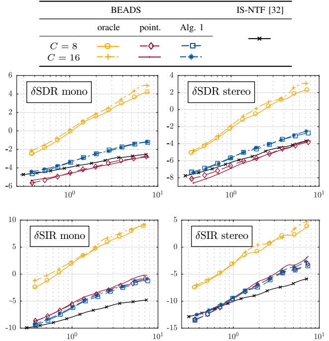
Fig. 2: BEADS for ISS on mono (left) or stereo (right) mixes. Metrics are \delta SDR (top) and \delta SIR (bottom). Units are kilobits/second/source (x-axis) and dB (y-axis).
