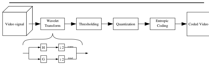
Figure 1. Encoder phases.
