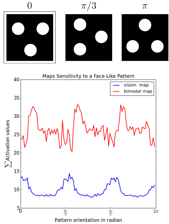
Fig. 3. Sensitivity to face-like patterns for certain orientations. When rotating the three dots pattern centered on the eye, the neural activity within the visual map and the bimodal map gets higher only to certain orientations.
