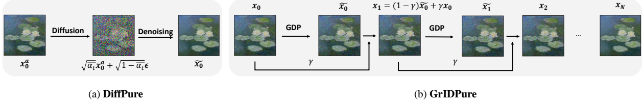
Figure 8. Framework of (a) DiffPure and our proposed (b) GrIDPure.
