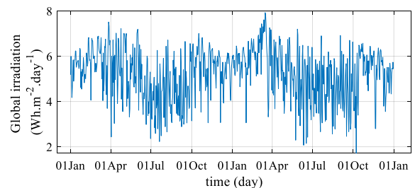
Fig. 3 Global daily irradiation over two years (2016-2017) of Yeripao site.
