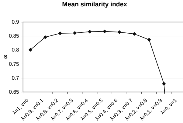
Fig. 9. Mean similarity indices obtained for different values of the parameters \lambda and \nu attached to the trade-off between the data term F_C and the spatial relations force F_R in Equation 17. With \lambda + \nu = 1 , \lambda and \nu vary between 0 and 1. The similarity is very stable for \lambda \in [0.3; 0.8] (and thus \nu \in [0.2; 0.7] ), the difference being smaller than 0.01. Outside this interval, the similarity is strongly decreased (the value corresponding to \lambda = 0 is S = 0 but is not shown to facilitate visualization).
