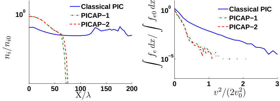
Figure 21: Plasma expansion test case. Simulation 4: space and time under-resolved case: \Delta x = 4\lambda and \Delta t = 3\omega_i^{-1} and small number of particles (1000 particles per mesh and per species). Ion density as a function of position in log scale (left) and electron velocity distribution as a function of v^2/(2v_0^2) (right) with Classical PIC and PICAP schemes, at time t = 30\omega_i^{-1} .
