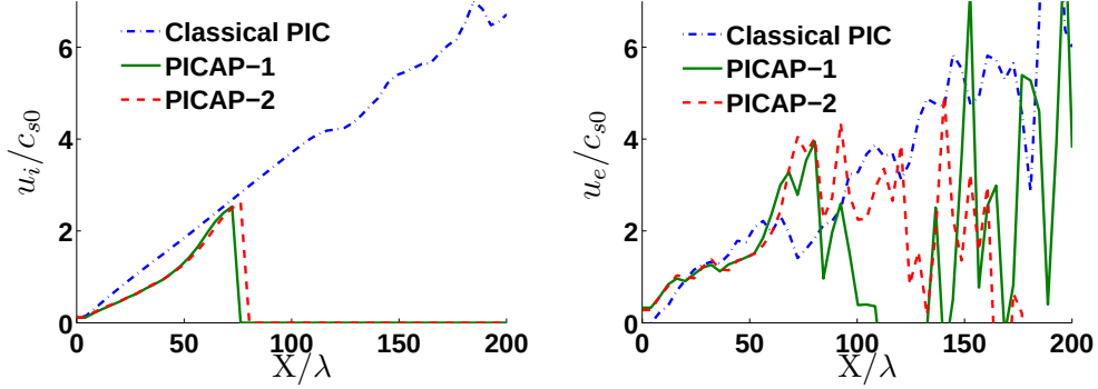
Figure 22: Plasma expansion test case. Simulation 4: space and time under-resolved case: \Delta x = 4\lambda and \Delta t = 3\omega_i^{-1} and small number of particles (1000 particles per mesh and per species). Ion and electron mean velocities as functions of position, with Classical PIC, PICAP-1 and PICAP-2 schemes, at time t = 30\omega_i^{-1} ( c_{s0} = \sqrt{k_B T_{e0}/m_i} ).
