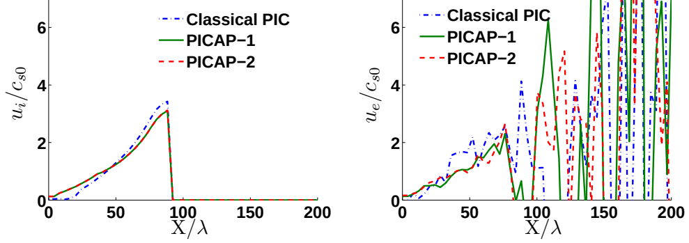
Figure 15: Plasma expansion test case. Simulation 2: space under-resolved and time resolved case: \Delta x = 4\lambda and \Delta t = 0.05\omega^{-1} . Ion and Electron mean velocities as functions of position, with Classical PIC, PICAP-1 and PICAP-2 schemes, at time t = 30\omega_i^{-1} ( c_{s0} = \sqrt{k_B T_{e0}/m_i} ).
