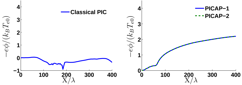
Figure 16: Plasma expansion test case. Simulation 3: space and time under-resolved case: \Delta x = 4\lambda and \Delta t = 3\omega^{-1} . Electric potential as a function of position, with Classical PIC scheme (left) and PICAP schemes (right), at time t = 30\omega_i^{-1} .
