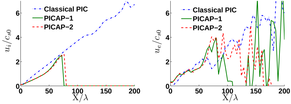
Figure 19: Plasma expansion test case. Simulation 3: space and time under-resolved case: \Delta x = 4\lambda and \Delta t = 3\omega_i^{-1} . Ion and Electron mean velocities as functions of position, with Classical PIC, PICAP-1 and PICAP-2 schemes, at time t = 30\omega_i^{-1} ( c_{s0} = \sqrt{k_B T_{e0}/m_i} ).
