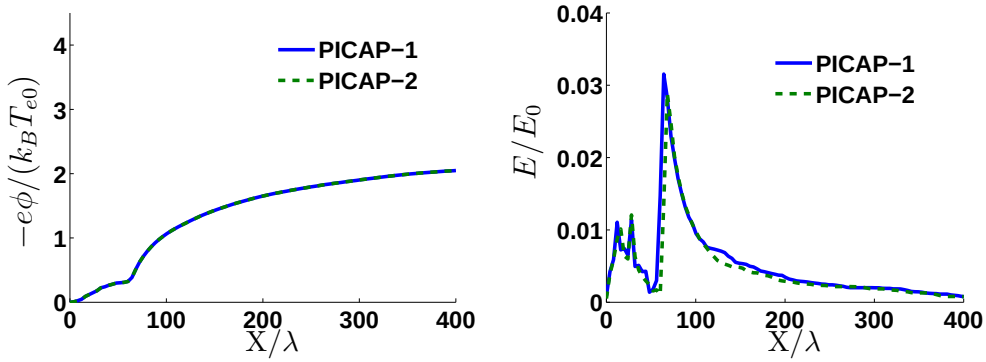
Figure 20: Plasma expansion test case. Simulation 4: space and time under-resolved case: \Delta x = 4\lambda and \Delta t = 3\omega_i^{-1} and small number of particles (1000 particles per mesh and per species). Electric potential (left) and electric field (right) as a function of position with PICAP schemes at time t = 30\omega_i^{-1} .
