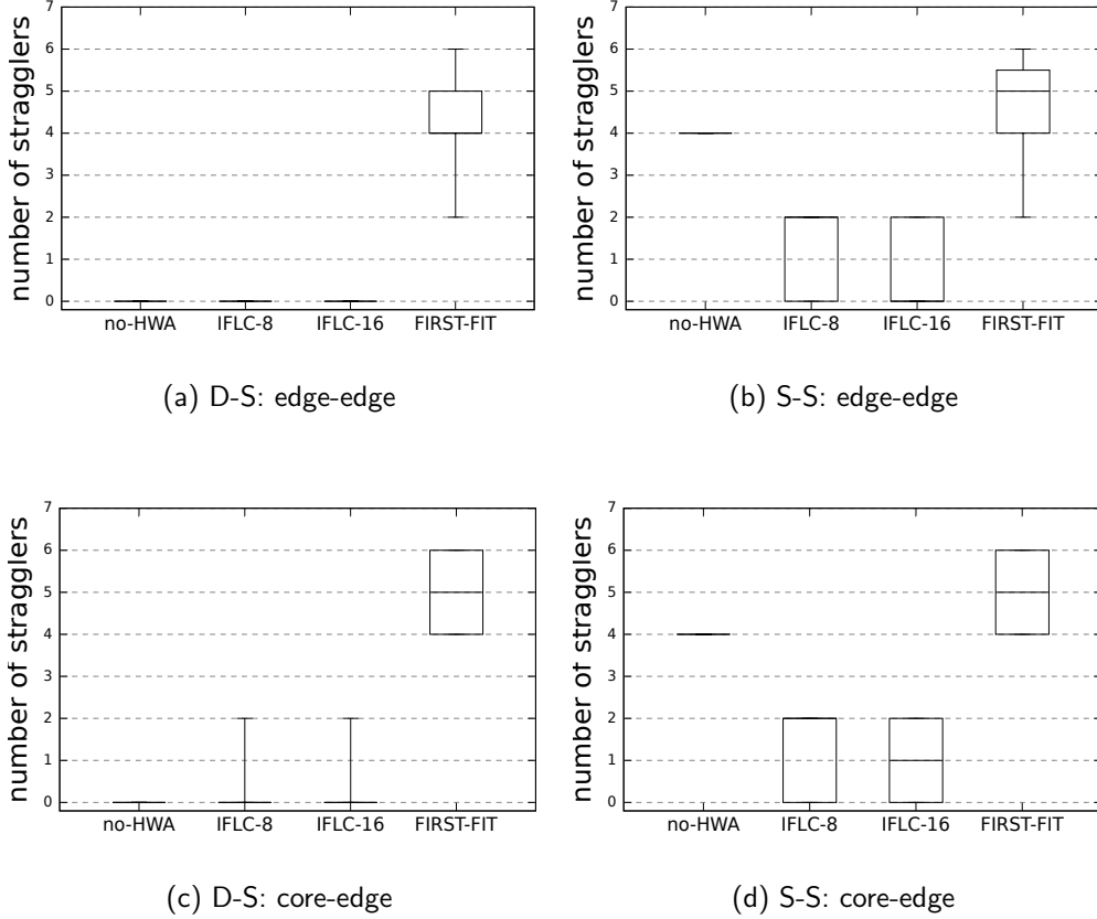
Figure 7: Distribution of the number of stragglers.
