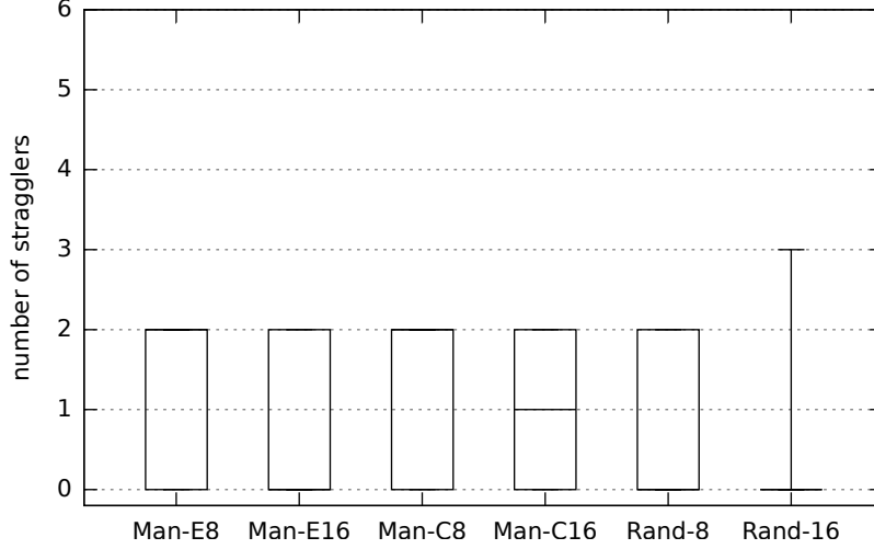
Figure 12: Distribution of the number of stragglers AIFs using IFLC: S-S case.
