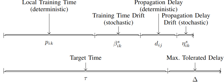
Figure 3: E2E training time ( \chi ) model components and threshold.
