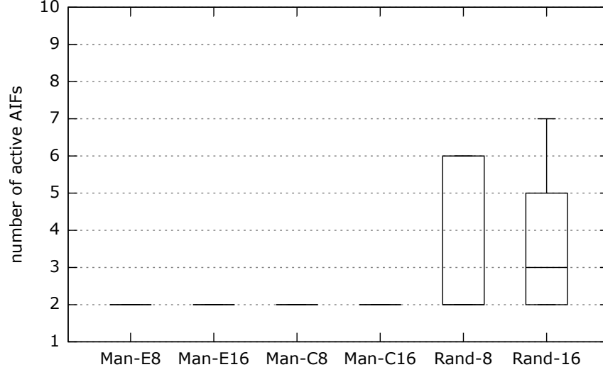
Figure 14: Distribution of the number of active AIFs using IFLC: S-S case.
