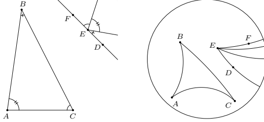
Fig. 15: Triangle postulate (Postulate 3).
