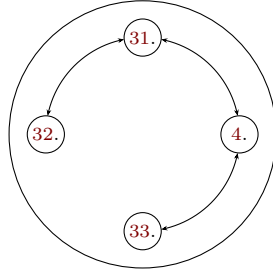
Fig. 51: Overview of the proofs of Sec. 7.2.
