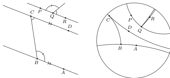
Fig. 22: Consecutive interior angles postulate (Postulate 8).
