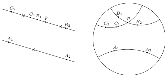
Fig. 14: Playfair's postulate (Postulate 2).
