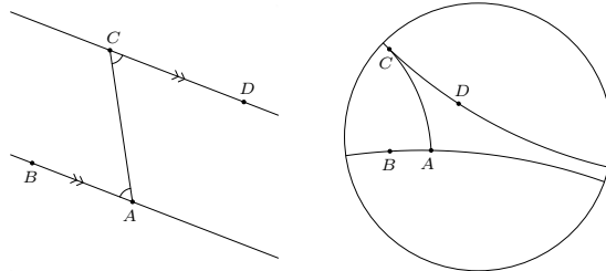
Fig. 21: Alternate interior angles postulate (Postulate 7).
