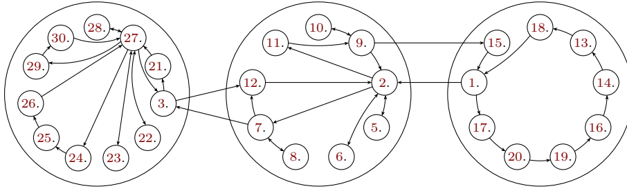
Fig. 47: Overview of the proofs.
