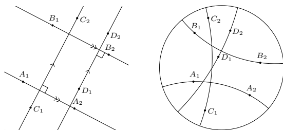
Fig. 25: Postulate of parallelism of perpendicular transversals (Postulate 10).
