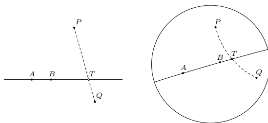
Fig. 8: Definition of TS.
