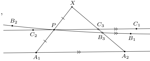
Fig. 30: Postulate 6 implies Postulate 2.
