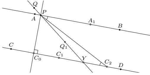
Fig. 50: Assuming Axiom 4, Postulate 7 implies Postulate 13.
