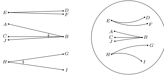
Fig. 10: Definition of SumA.
