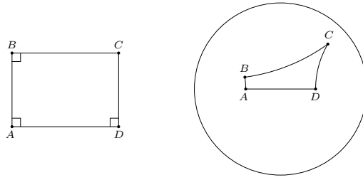
Fig. 45: Definition of Lambert.
