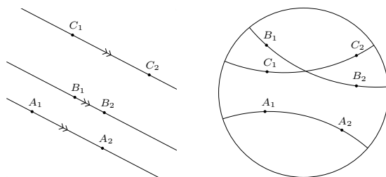
Fig. 19: Postulate of transitivity of parallelism (Postulate 5).
