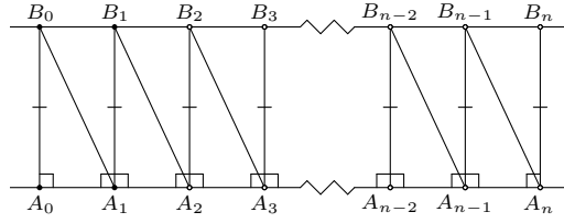
Fig. 52: Considered points in Theorem 22.18 of [Mar98].
