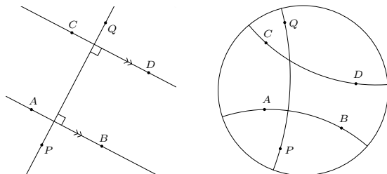
Fig. 24: Perpendicular transversal postulate (Postulate 9).
