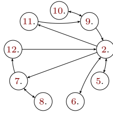
Fig. 29: Overview of the proofs of Sec. 4.
