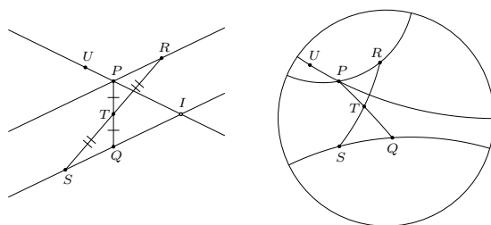
Fig. 36: Strong parallel postulate (Postulate 18).
