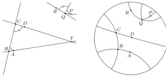
Fig. 38: Euclid’s parallel postulate (Postulate 20).
