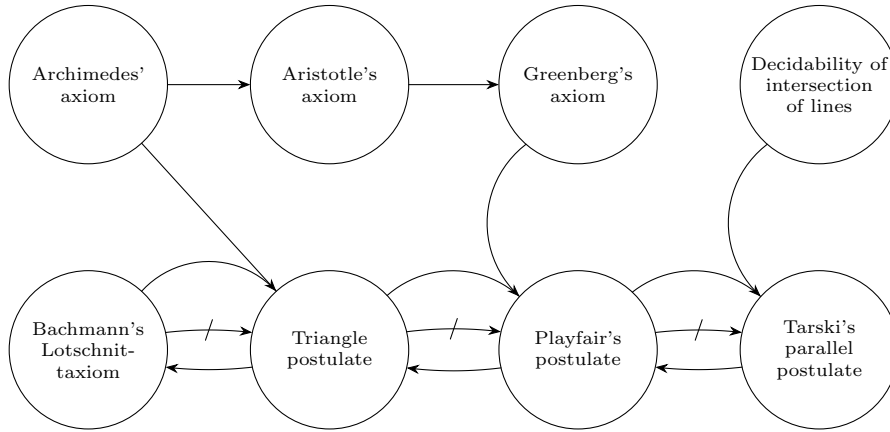
Fig. 5: Graphical summary of the independence results from Sections 3.1.1-3.1.3.
