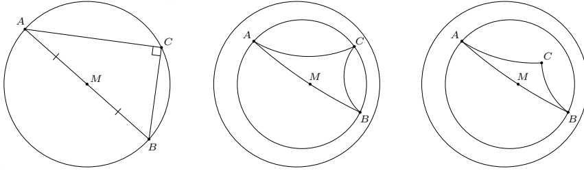
Fig. 43: Thales' postulate (Postulate 24), Thales' converse postulate (Postulate 25) and existential Thales' postulate (Postulate 26).
