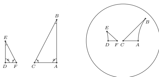
Fig. 42: Postulate of existence of similar but non-congruent triangles (Postulate 23).
