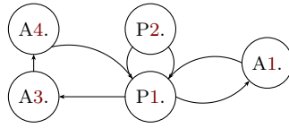
Fig. 49: Overview of the proof of the equivalence between Axiom 1, Axiom 3 and Axiom 4.
