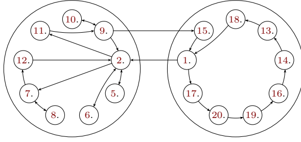
Fig. 39: Overview of the proofs of Sec. 5.
