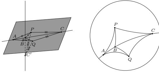
Fig. 4: Upper dimensional axiom A9.
