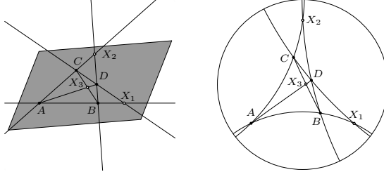
Fig. 6: Definition of Coplanar.
