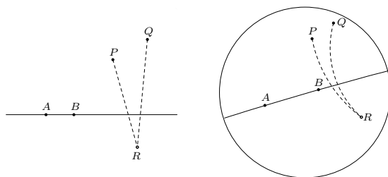
Fig. 9: Definition of OS.
