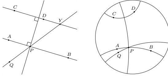
Fig. 32: Alternative Proclus' postulate (Postulate 14).
