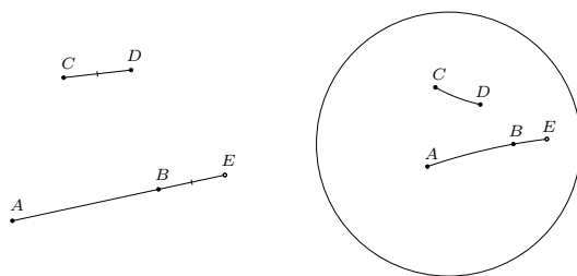
Fig. 1: Axiom of segment construction A4.
