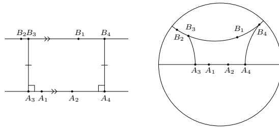
Fig. 26: Universal Posidonius' postulate (Postulate 11).
