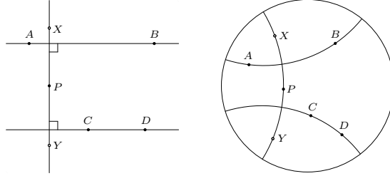
Fig. 27: Definition of \text{Perp2} .
