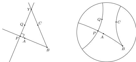
Fig. 34: Inverse projection postulate (Postulate 16).
