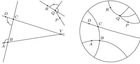
Fig. 37: Alternative strong parallel postulate (Postulate 19).
