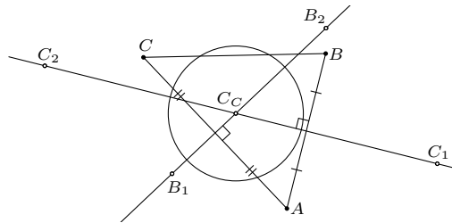
Fig. 40: Axiom 1 and Postulate 9 imply Postulate 15.
