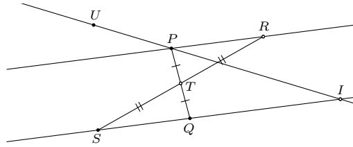
Fig. 41: Postulate 18 implies Axiom 1.
