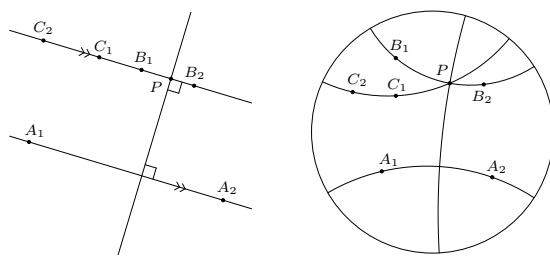
Fig. 28: Alternative Playfair's postulate (Postulate 12).
