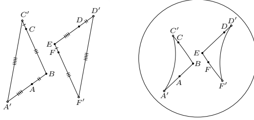
Fig. 7: Definition of CongA.
