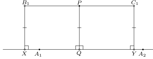
Fig. 55: Postulate 7 implies Postulate 3.
