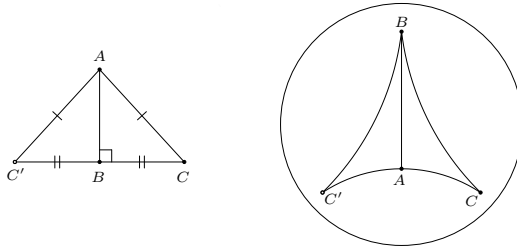
Fig. 11: Definition of \text{Per} .
