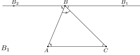
Fig. 48: Postulate 7 implies Postulate 3.
