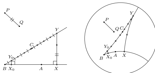
Fig. 53: Axiom 2 implies Axiom 3.
