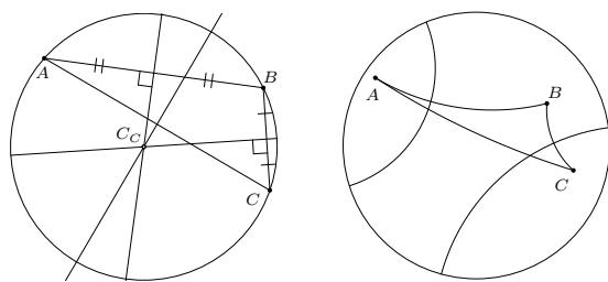
Fig. 33: Triangle circumscription principle (Postulate 15).
