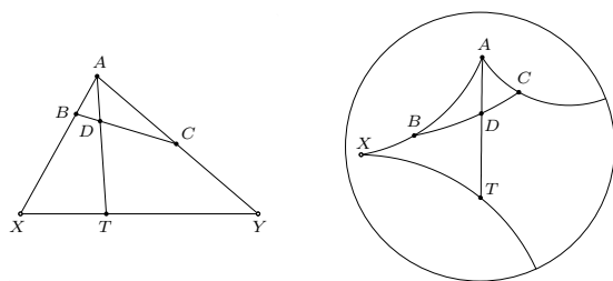
Fig. 13: Tarski's parallel postulate (Postulate 1).
