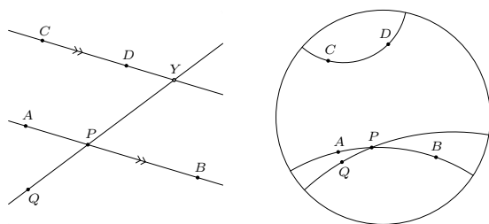
Fig. 31: Proclus' postulate (Postulate 13).
