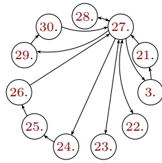
Fig. 46: Overview of the proofs of Sec. 6.
