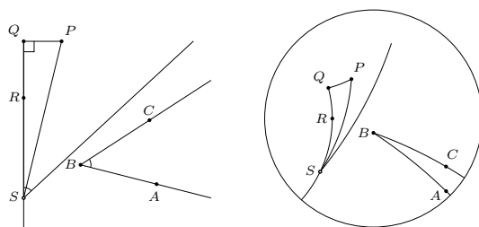
Fig. 18: Greenberg's axiom (Axiom 4).
