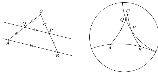
Fig. 20: Midpoint converse postulate (Postulate 6).
