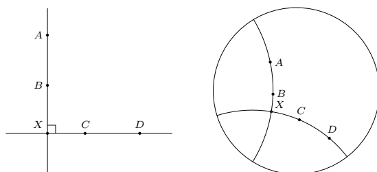
Fig. 23: Definition of \text{Perp\_at} .
