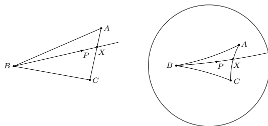
Fig. 12: Definition of \text{InAngle} .
