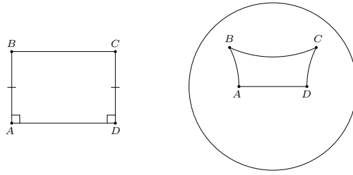
Fig. 44: Definition of Saccheri.
