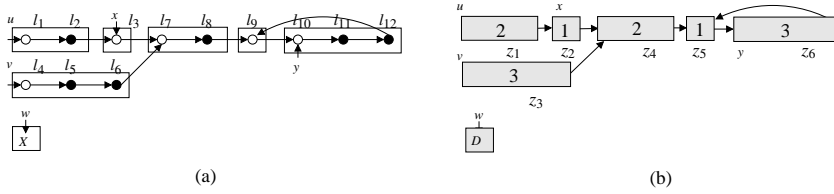
Fig. 4 SSG and Concretization
