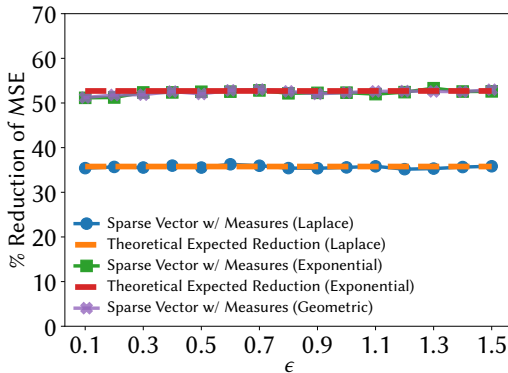
(a) SVT with Gap with Measures, kosarak.
