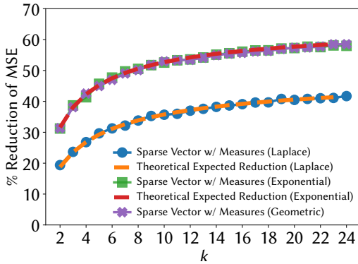
(a) SVT with Gap with Measures, BMS-POS.
