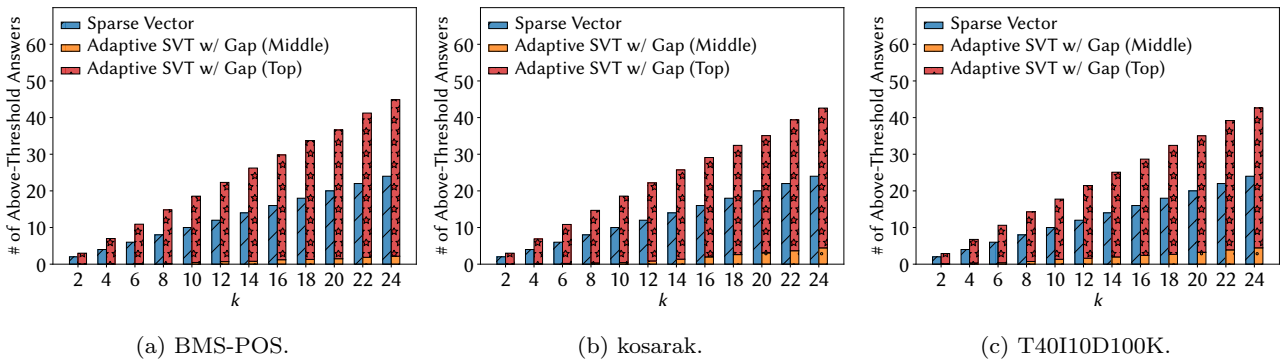
Fig. 4: # of queries answered by SVT and Adaptive SVT with Gap under different k 's for monotonic queries. Privacy budget \epsilon = 0.7 and x -axis: k .
