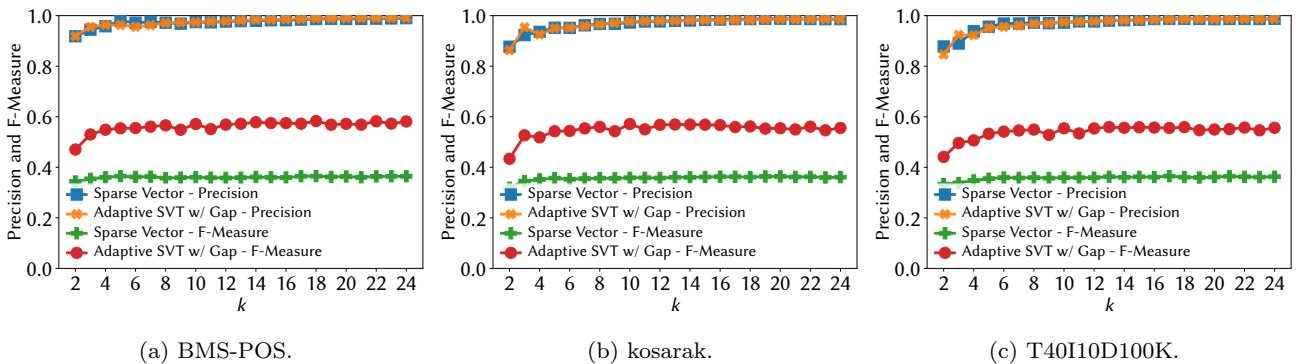
Fig. 5: Precision and F-Measure of SVT and Adaptive SVT with Gap under different k 's for monotonic queries. Privacy budget \epsilon = 0.7 and x -axis: k .
