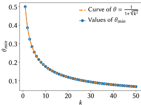
Fig. 1: The blue dots are values of \theta_{\min} = \text{argmin}(\frac{e^{\theta\epsilon}}{(e^{\theta\epsilon} - 1)^2} + \frac{e^{(1-\theta)\epsilon/k}}{(e^{(1-\theta)\epsilon/k} - 1)^2}) for k from 1 to 50. The orange curve is the function \theta = 1/(1 + \sqrt[3]{k^2}) .
