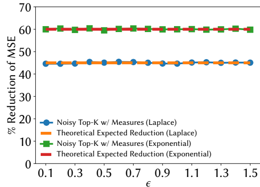
(b) Noisy Top-K with Gap with Measures, kosarak.
