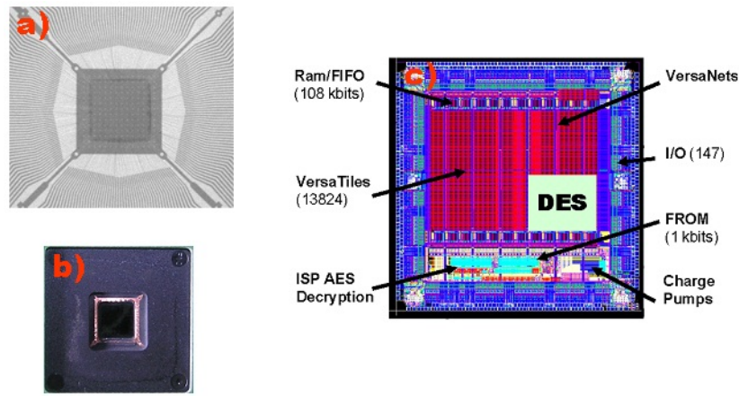
Fig. 2. Different view and informations about the FPGA Actel Proasic3e a) x-ray image b) Picture of the FPGA open from the backside c) Layout informations [20] with location of the DES implementation
