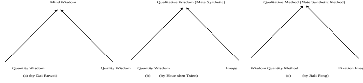
Fig. 2. (a)Quantity Wisdom \otimes Quality Wisdom \Rightarrow Mind Wisdom (by Dai Ruwei) (b) Quantity Wisdom \otimes Image Wisdom \Rightarrow Qualitative Wisdom (Mate Synthetic Wisdom) (by Hsue-shen Tsien) (c) Quantity Method \otimes Fixation Image \Rightarrow Qualitative Method (Mate Synthetic Method) (by Jiali Feng)
