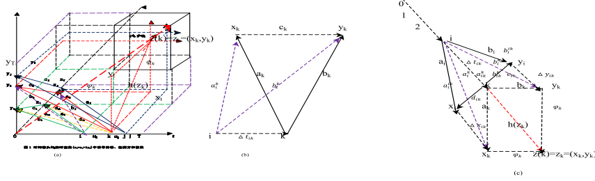
Fig. 4. (a) Category induced by arrows \{(\Delta t, \Delta x, \Delta y)\} Fig.4(b) Cone of arrows F = \{(a_k, b_k, c_k)\} , Fig.4(c) Pullback (a_k, b_k) of position mapping (\varphi_k, \varphi_k)
