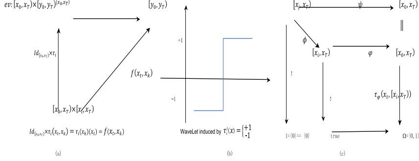
Fig. 5. (a) the Cartesian Closed Category induced by function f(x_t, x_k) and \tau_i(x_k) (b) Quality
