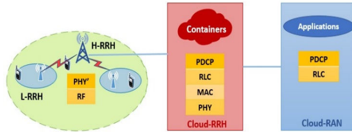
Fig. 1. Proposed C-RAN architecture
