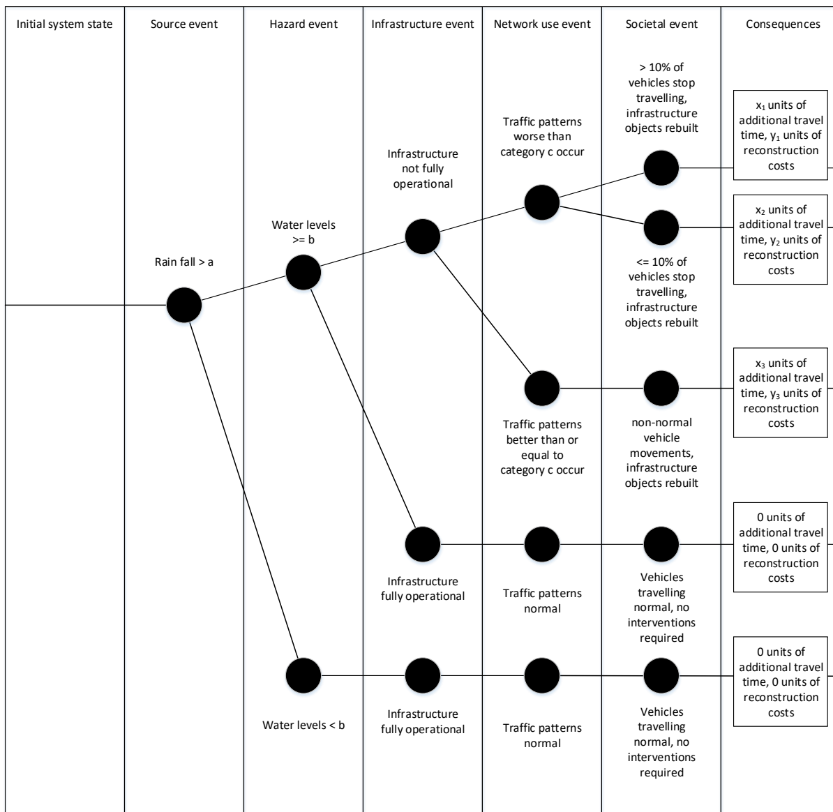
Figure III Example of a simple event tree for the definition of scenarios (Adey et al. 2016)
