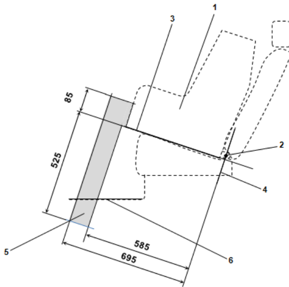
Figure 9 Side view of the i-Size support leg installation assessment volume for assessing compatibility of the i-Size seating positions with support legs of i-Size child restraint systems
