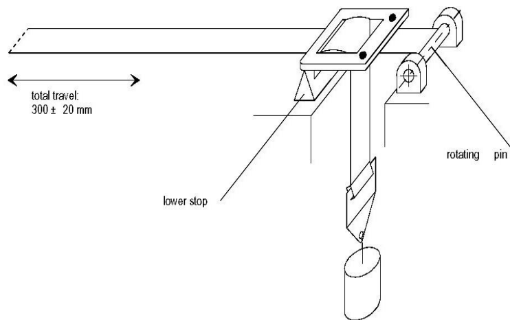
Example b Examples of test arrangements corresponding to the type of adjusting device
