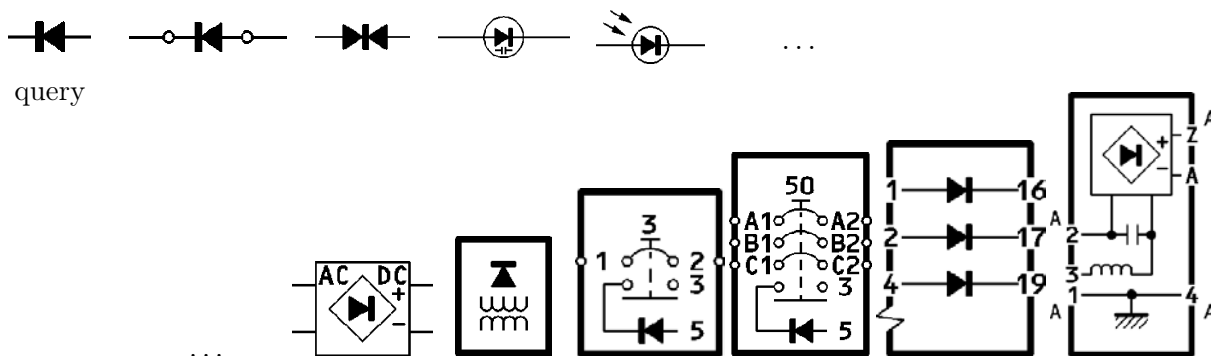
Figure 1.3: Selection of similar database symbols for a chosen query. The first symbol is considered to be a query symbol and remaining are ‘ground-truths’ associated with it. Ground-truth associated with a chosen query is not only concerned with similar visual overall appearance but also significant known parts within it, that may or may not be connected with other graphical elements and text.
