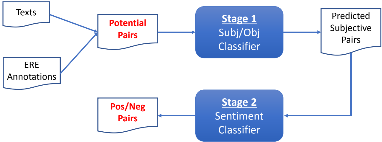
Figure 1: Two-Stage Classifier
