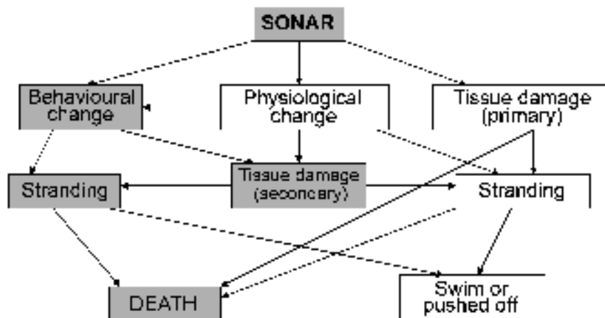
Figure 4. Potential mechanistic pathways by which beaked whales are affected by active sonar. (See Cox et al., 2006 for detailed discussion)
