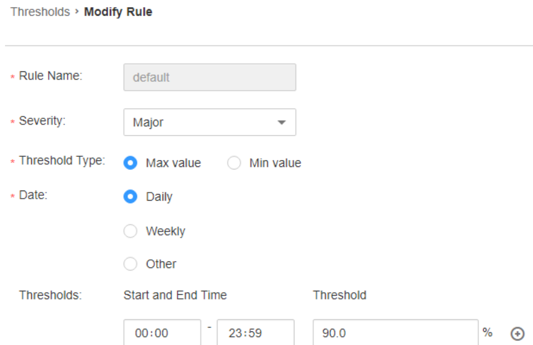
Figure 7-63 Setting an alarm threshold
