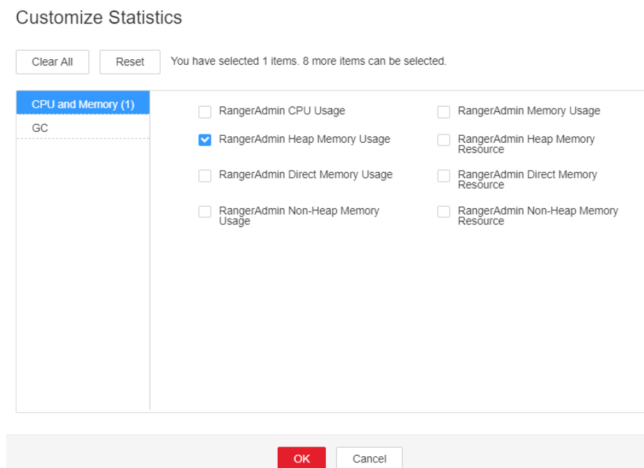
Figure 7-164 RangerAdmin heap memory usage
