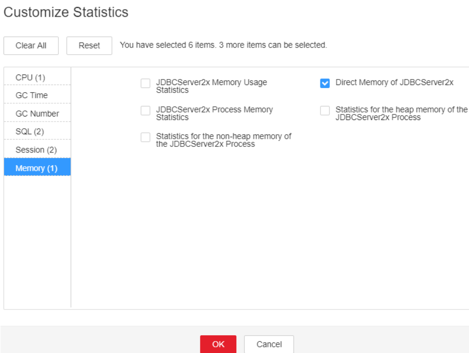
Figure 7-148 Direct Memory of JDBCServer2x
