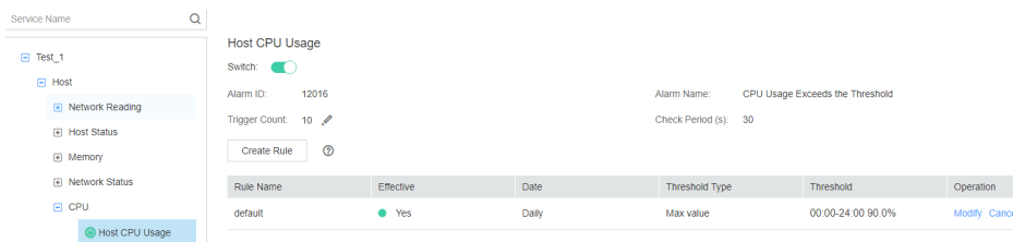
Figure 7-52 Setting alarm smoothing times
