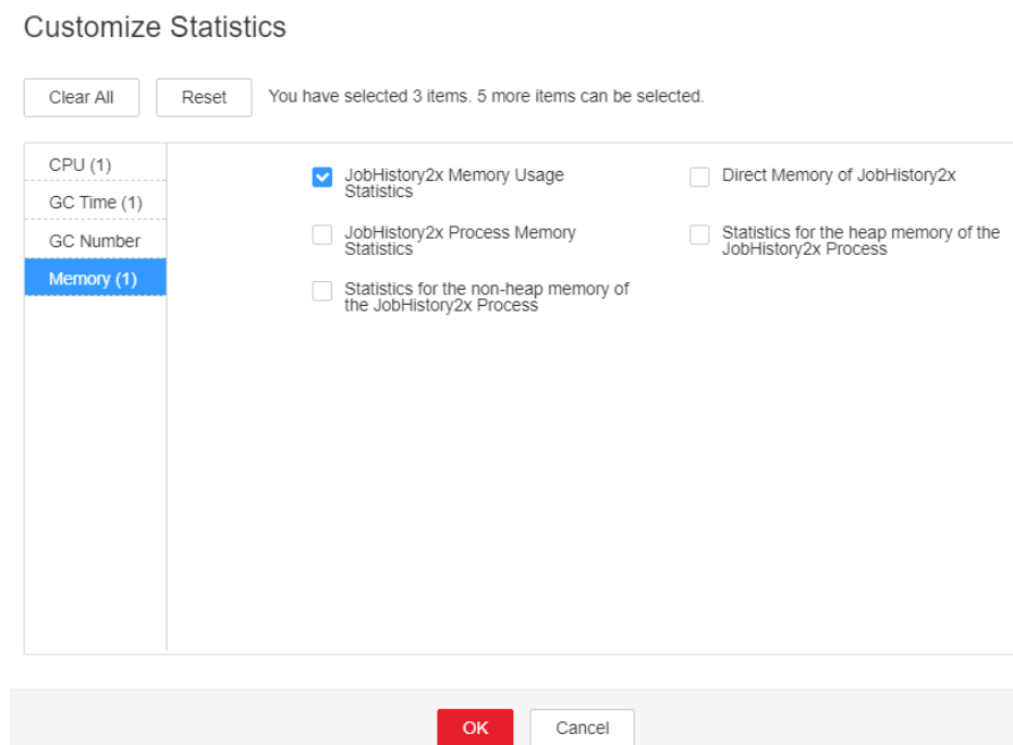
Figure 7-136 JobHistory2x Memory Usage Statistics
