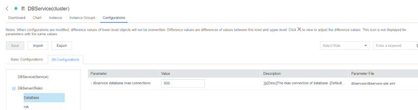
Figure 7-126 Setting the maximum number of database connections
