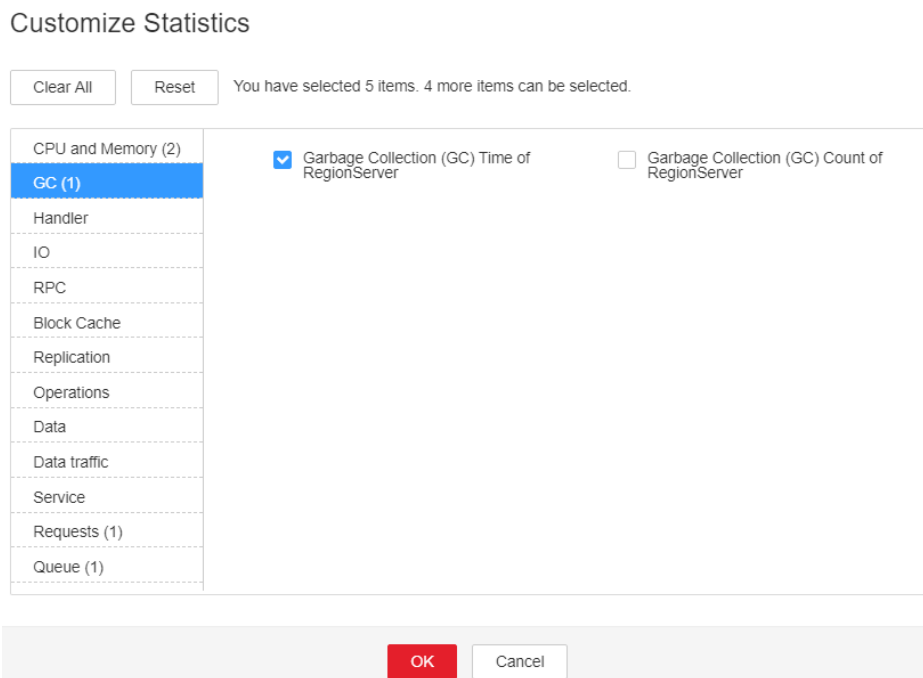
Figure 7-107 Garbage Collection (GC) Time of RegionServer
