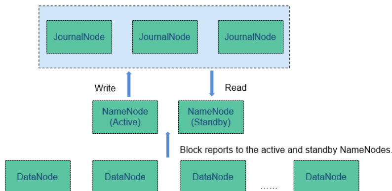
Figure 6-38 QJM-based HDFS architecture
