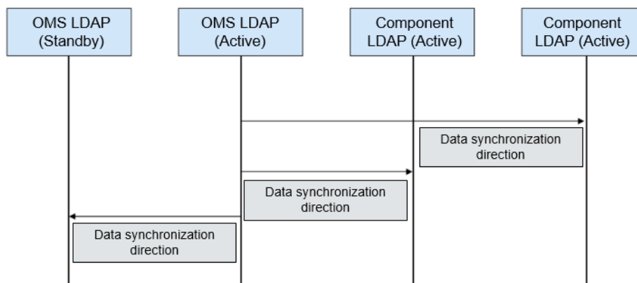
Figure 6-74 LDAP data synchronization
