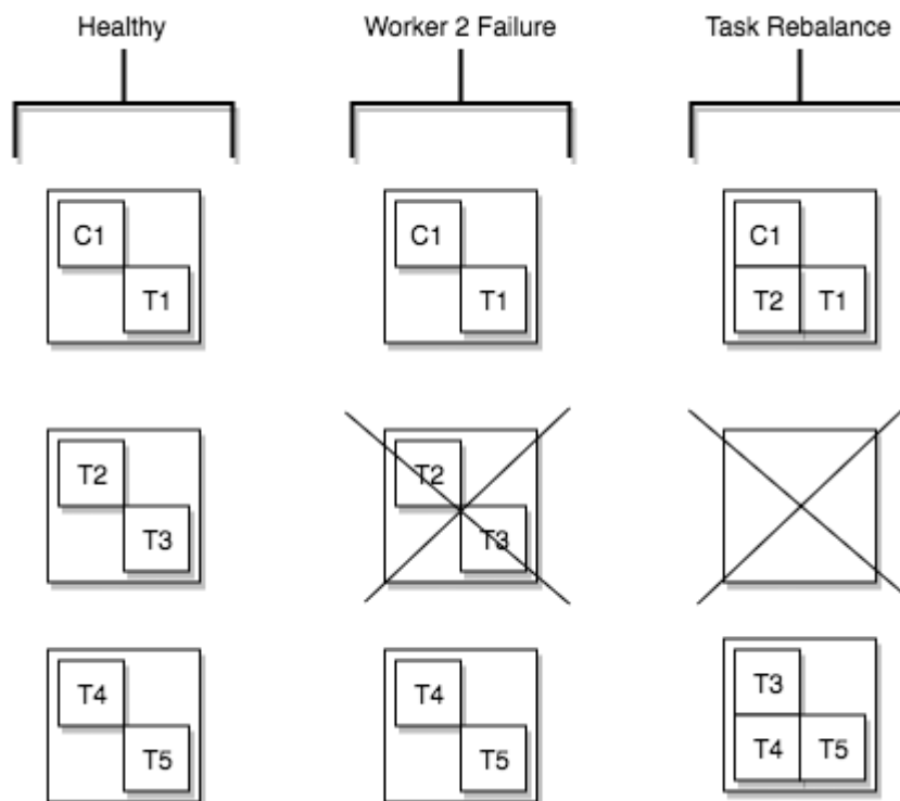
Figure 6-6 Rebalance of a task
