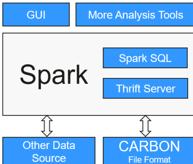
Figure 6-2 Basic architecture of CarbonData
