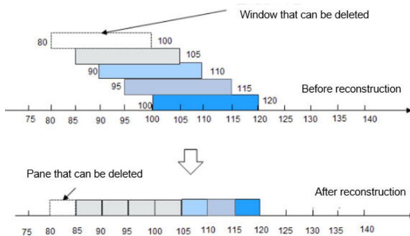
Figure 6-19 Deleting a window
