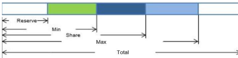
Figure 6-138 Resource scheduling policies
