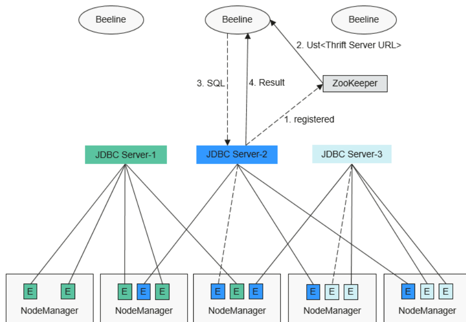
Figure 6-99 Spark JDBCServer HA
