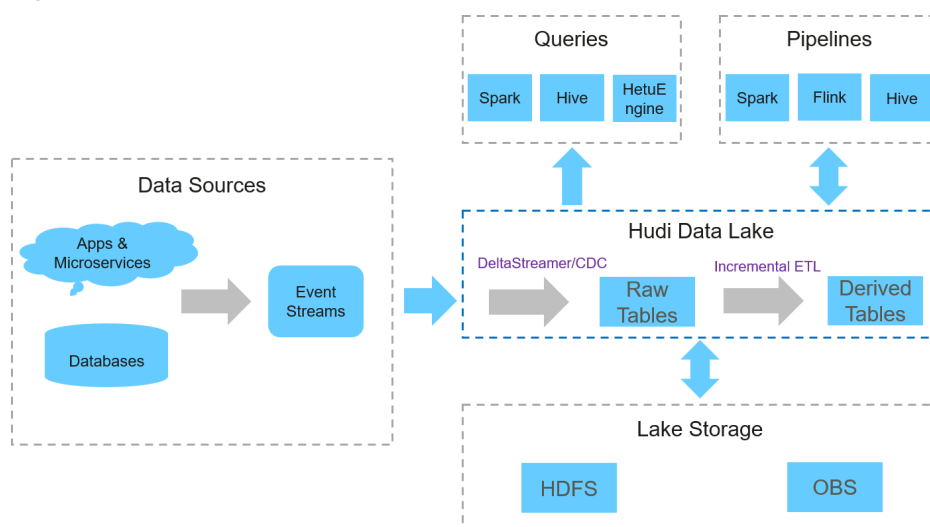
Figure 6-61 Basic architecture of Hudi
