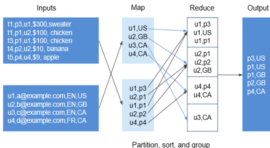
Figure 6-44 Data transmission in the non-colocation scenario
