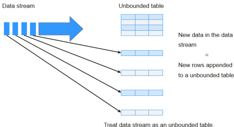
Figure 6-112 Unbounded table of Structured Streaming
