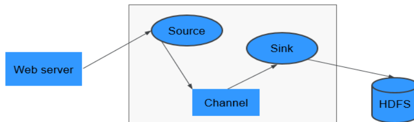
Figure 6-23 Flume-NG architecture
