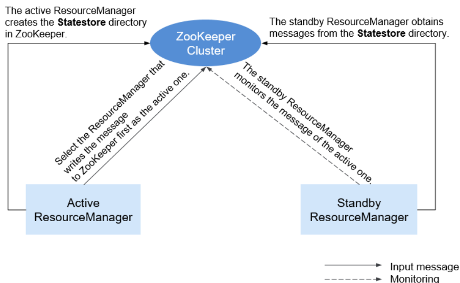
Figure 6-135 Relationship Between ZooKeeper and YARN
