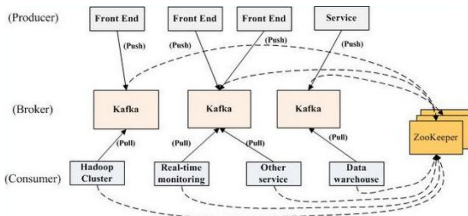
Figure 6-145 Relationship between ZooKeeper and Kafka
