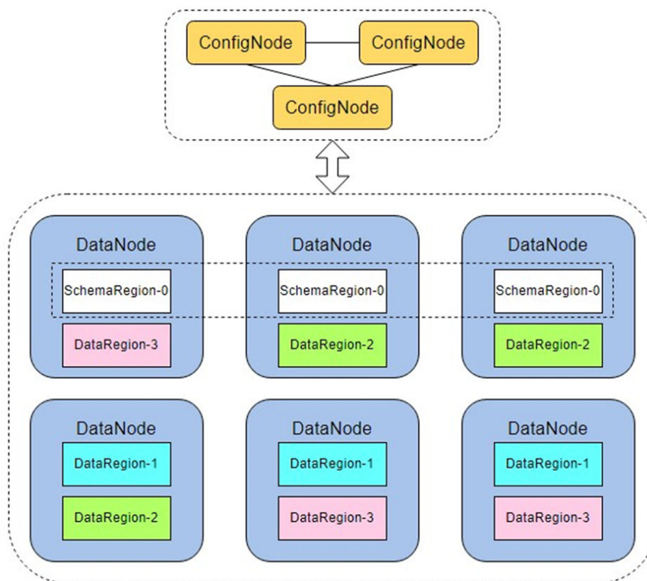
Figure 6-65 IoTDB distributed architecture
