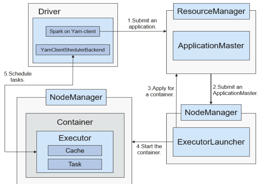
Figure 6-104 Spark on Yarn-client operation framework
