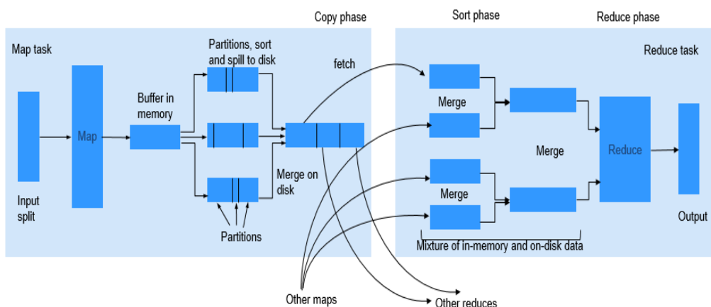
Figure 6-81 Job execution process
