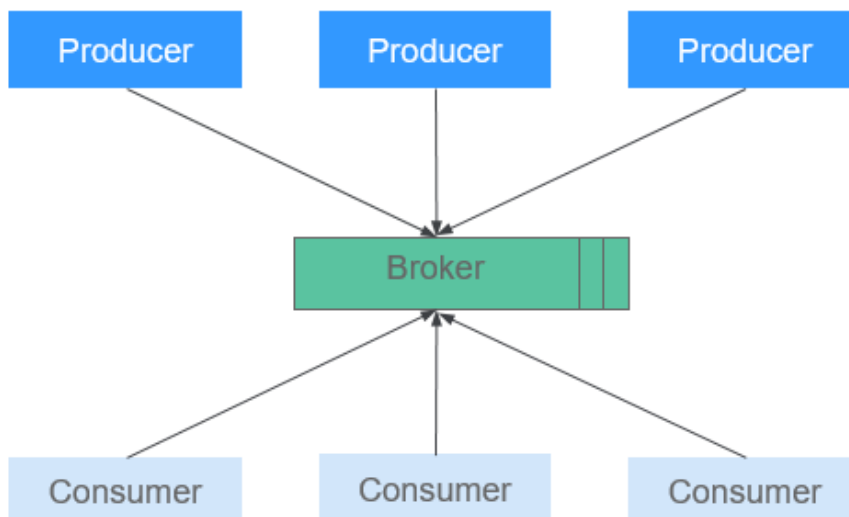
Figure 6-67 Kafka architecture
