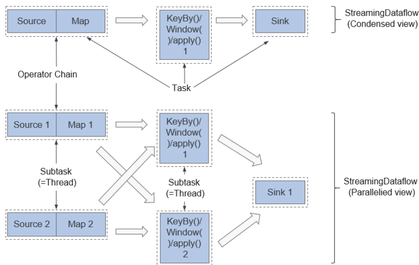
Figure 6-12 Operator chain
