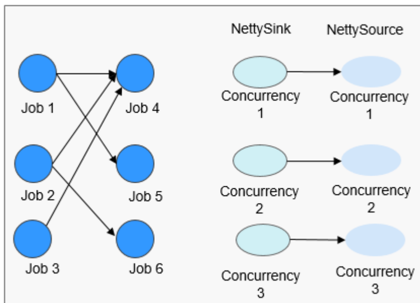
Figure 6-22 Relationship diagram
