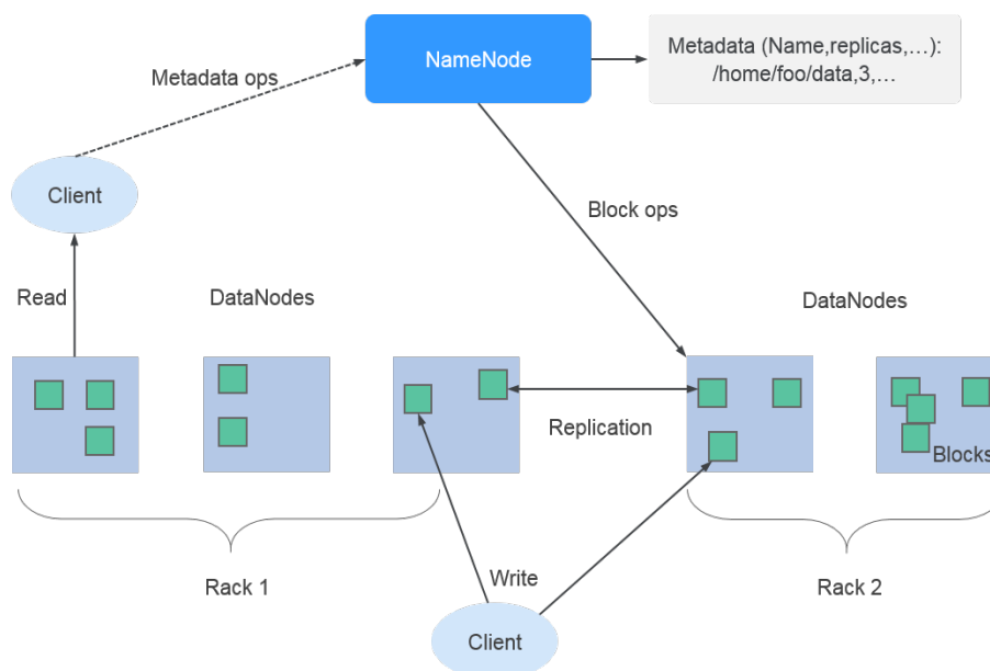
Figure 6-39 HDFS architecture
