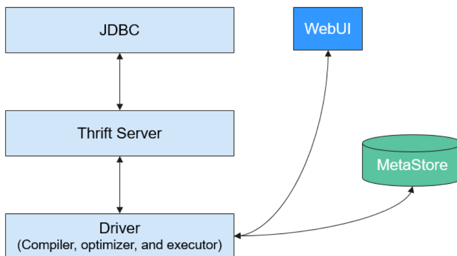
Figure 6-56 Hive framework
