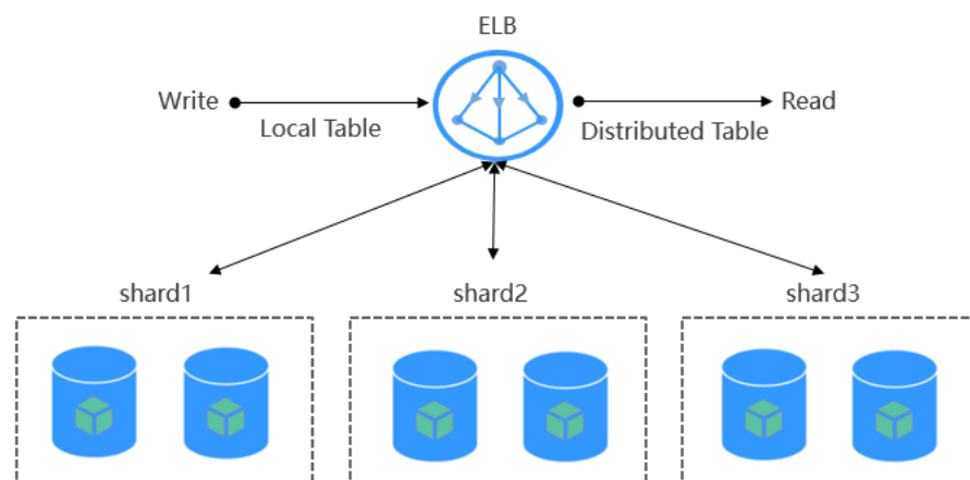
Figure 6-5 HA deployment architecture
