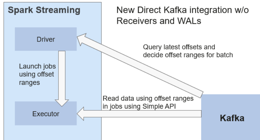
Figure 6-90 Data transmission through Direct Kafka API
