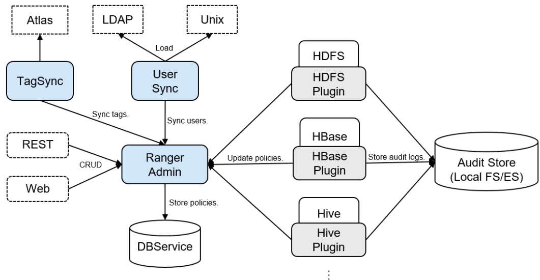
Figure 6-85 Ranger structure
