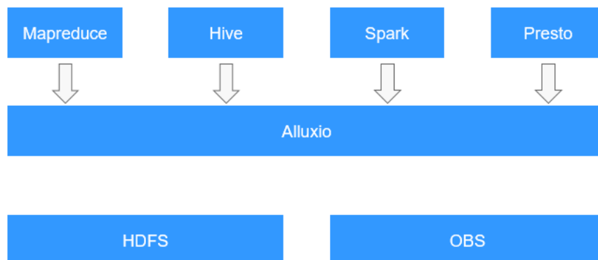
Figure 6-1 Alluxio architecture
