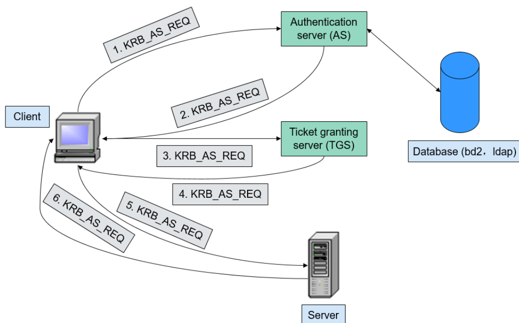
Figure 6-71 Authentication process
