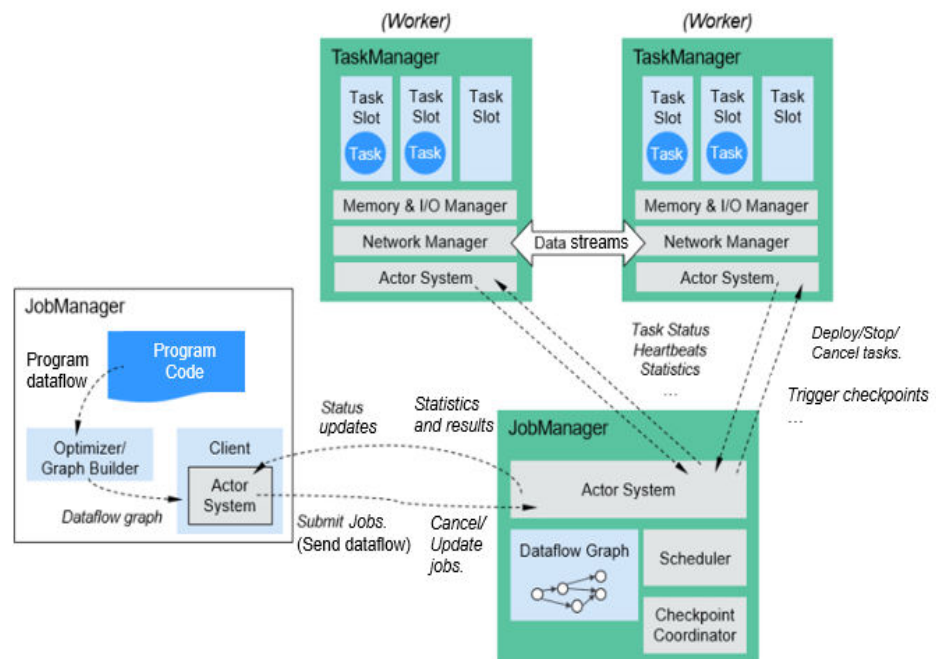
Figure 6-9 Flink architecture
