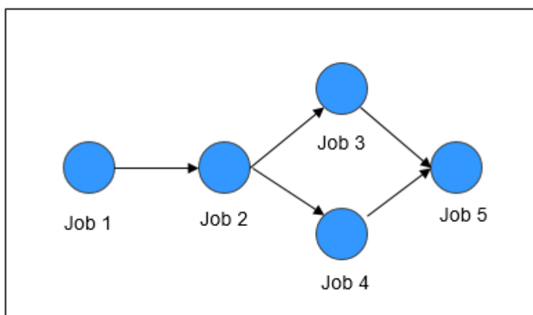
Figure 6-20 Job pipeline
