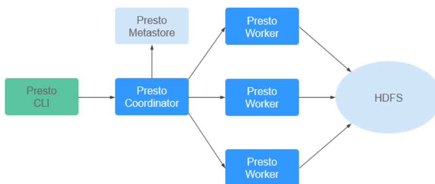
Figure 6-84 Presto architecture
