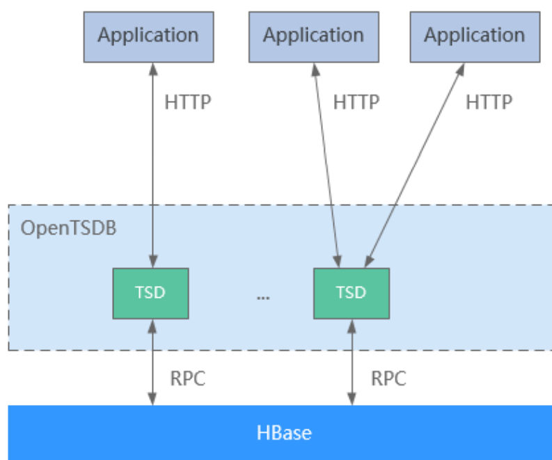
Figure 6-83 OpenTSDB architecture
