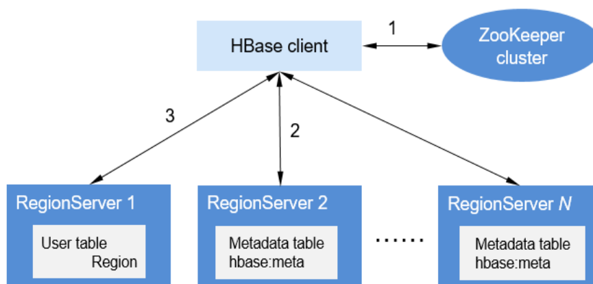
Figure 6-31 Data processing
