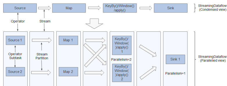
Figure 6-11 Operator
