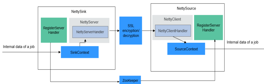
Figure 6-21 Job Pipeline
