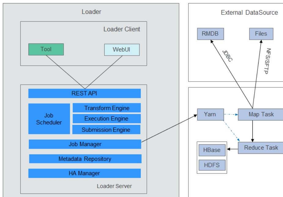
Figure 6-75 Loader model
