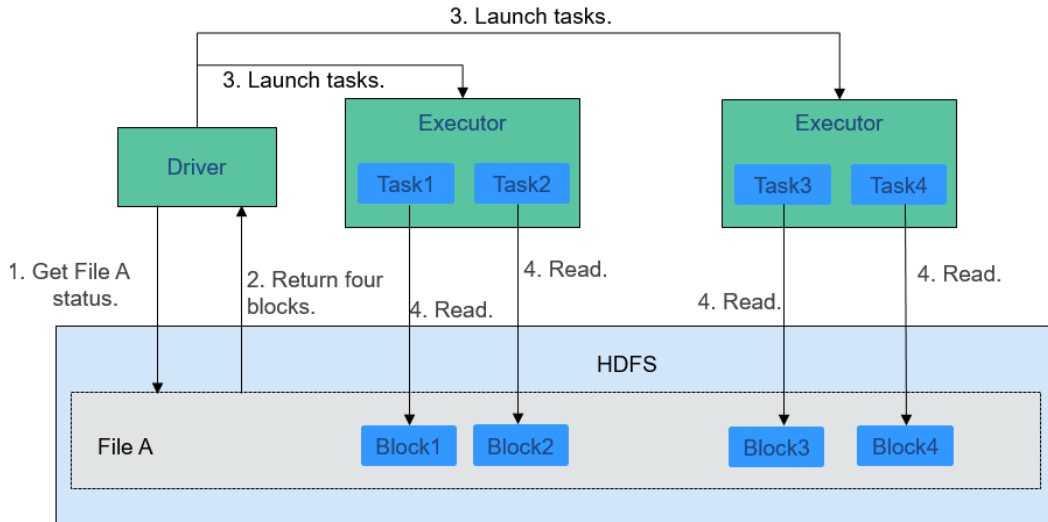
Figure 6-41 File reading process
