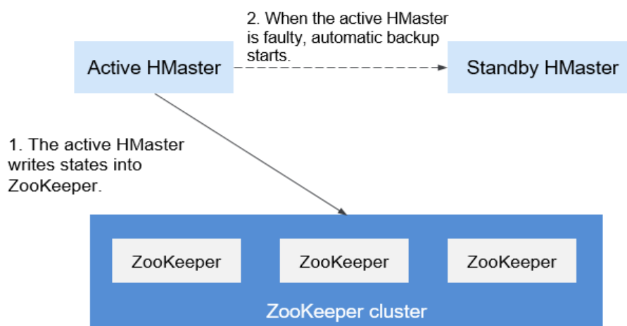
Figure 6-32 HMaster HA implementation architecture
