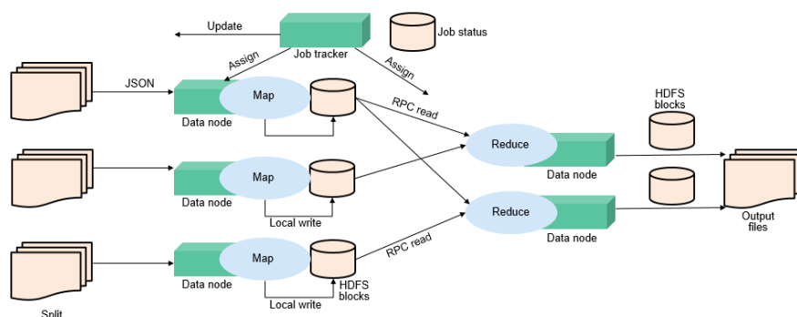
Figure 6-77 Distributed batch processing engine
