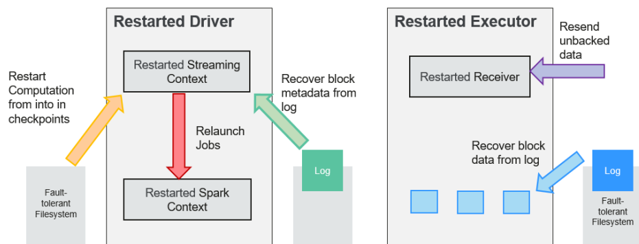
Figure 6-92 Computing recovery process
