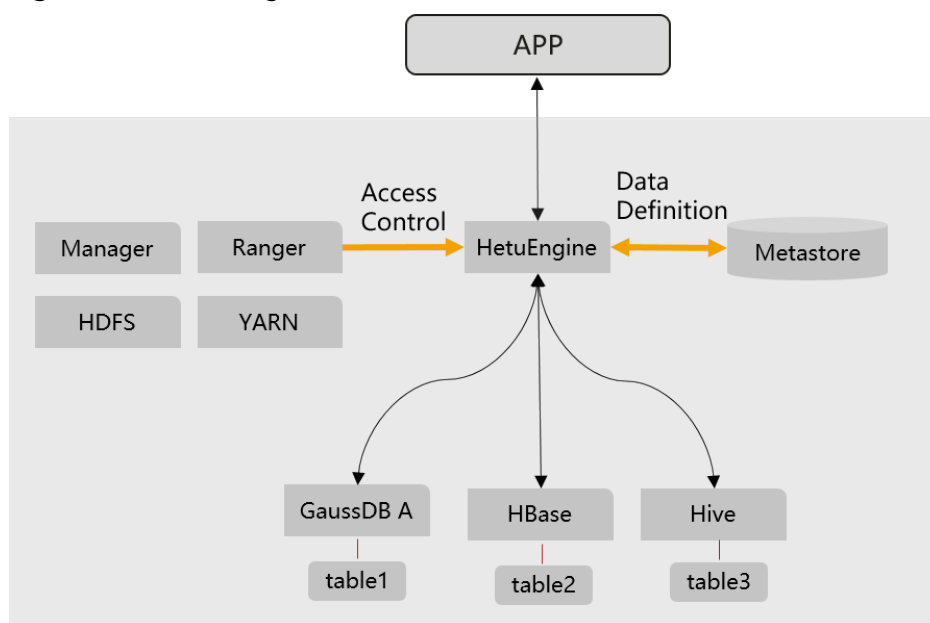
Figure 6-52 HetuEngine cross-source function
