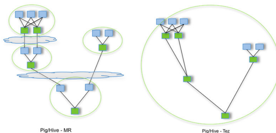
Figure 6-129 Processes for submitting tasks using Hive on MapReduce and Hive on Tez
