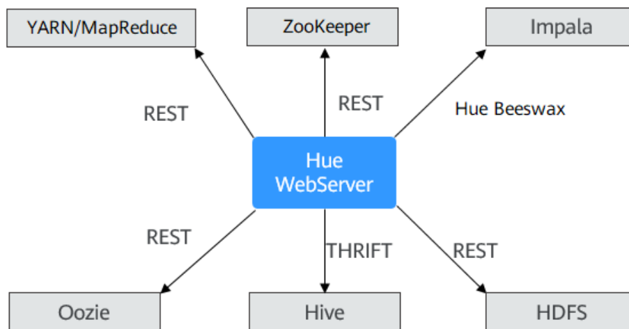
Figure 6-63 Hue and Hadoop clusters
