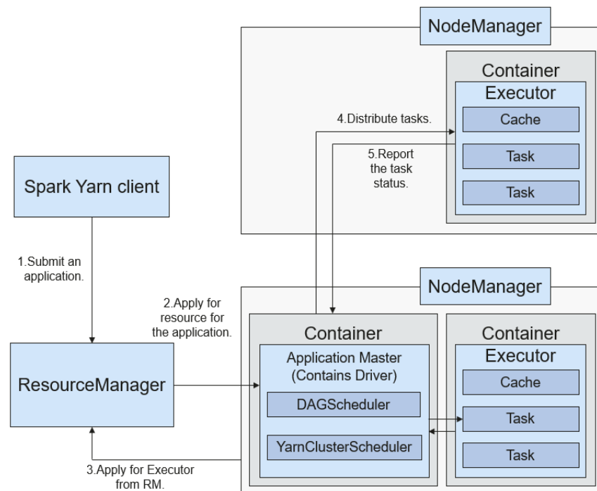
Figure 6-121 Spark on Yarn-cluster operation framework
