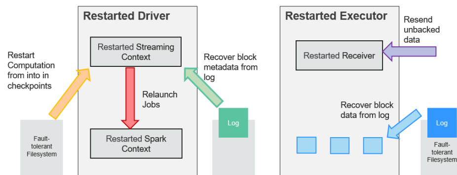
Figure 6-110 Computing recovery process
