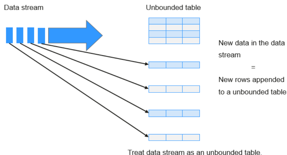
Figure 6-94 Unbounded table of Structured Streaming
