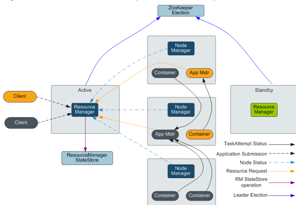
Figure 6-78 Basic architecture of Apache YARN and MapReduce
