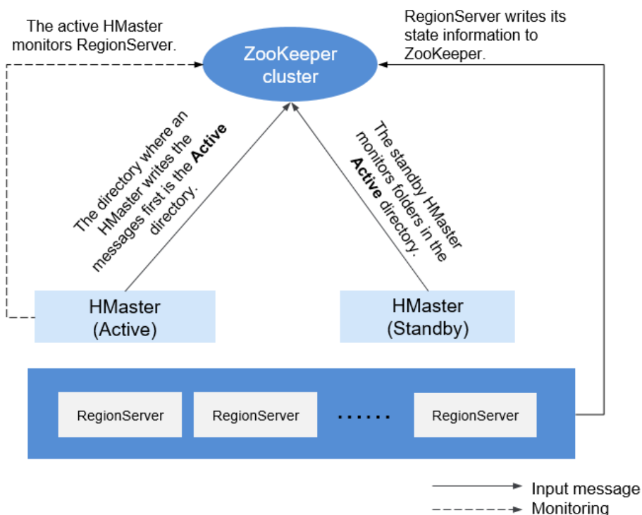
Figure 6-33 Relationship between ZooKeeper and HBase
