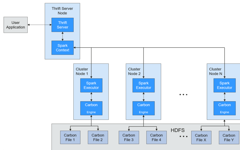
Figure 6-124 Topology of CarbonData
