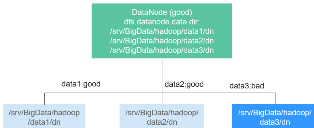
Figure 6-47 Item being set to 1
