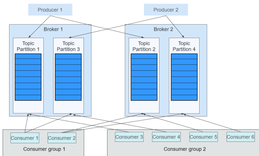
Figure 6-68 Relationships between Kafka modules
