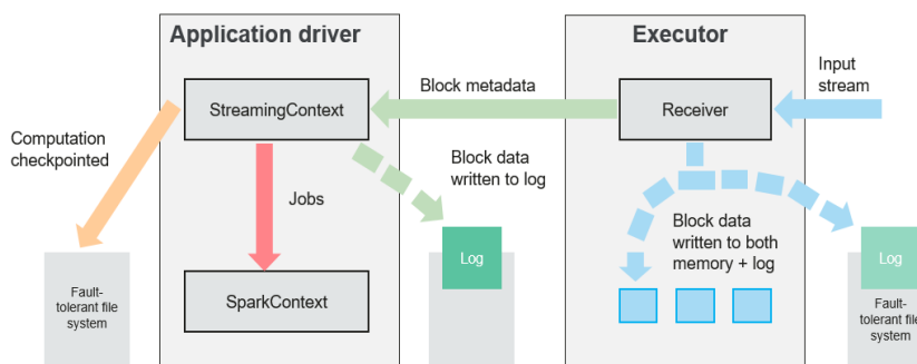
Figure 6-109 Data transfer lifecycle
