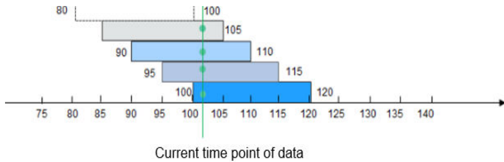
Figure 6-15 Original structure of a window
