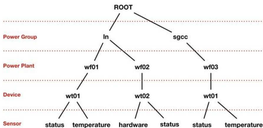
Figure 6-66 IoTDB data model
