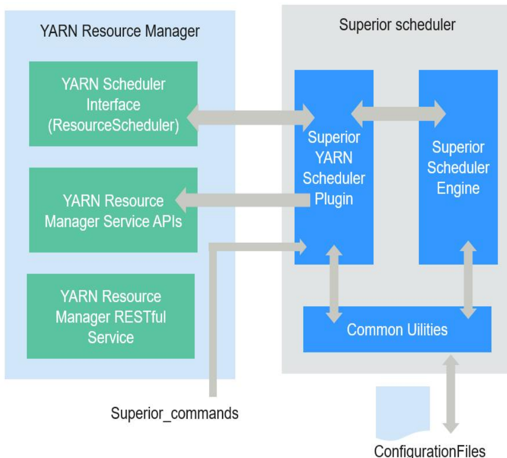
Figure 6-136 Internal architecture of Superior Scheduler
