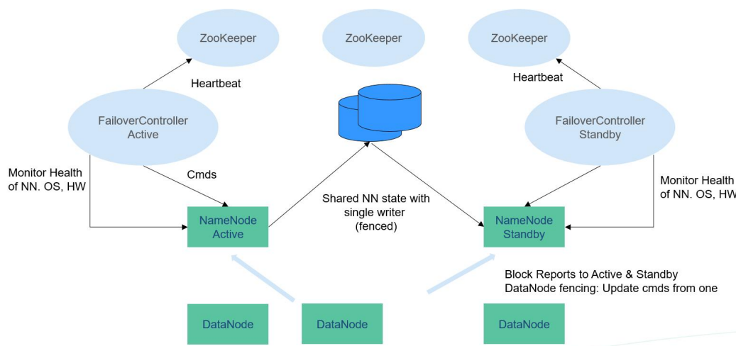
Figure 6-40 Typical HA deployment
