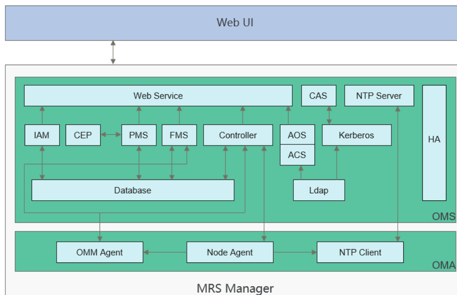
Figure 6-76 Manager logical architecture
