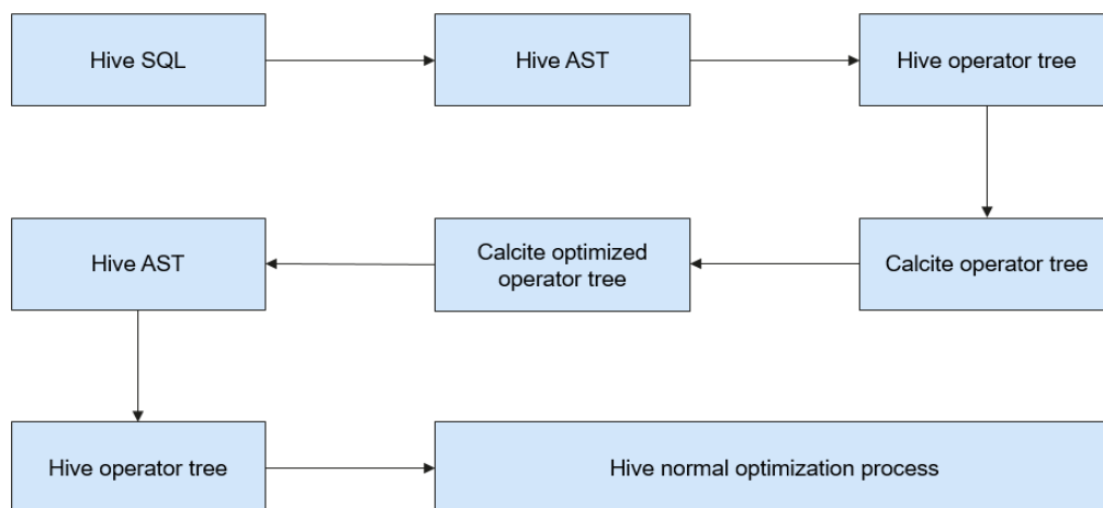
Figure 6-57 CBO Implementation process
