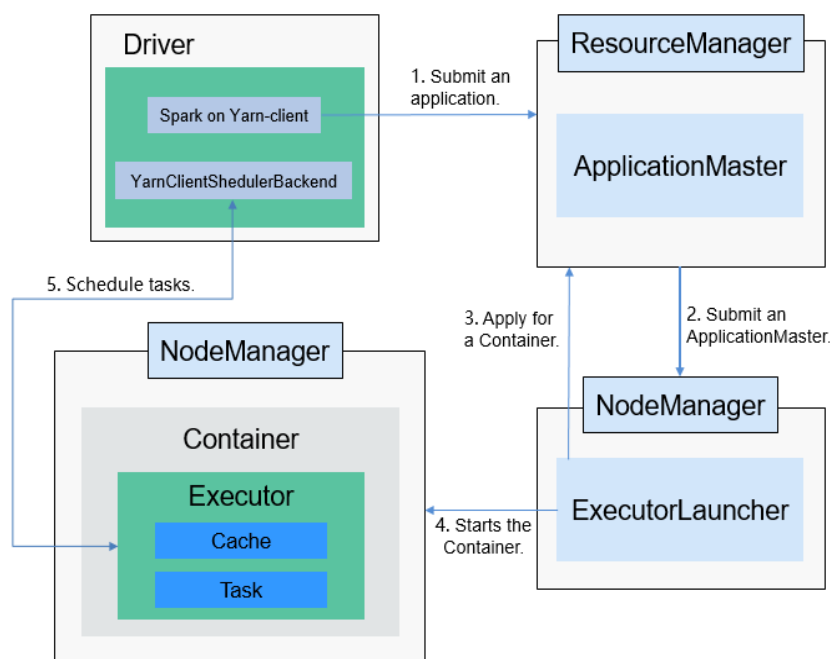
Figure 6-134 Spark on YARN-client operation framework
