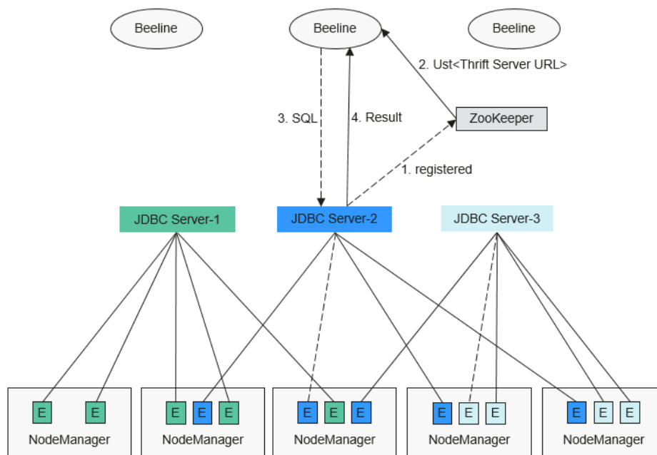
Figure 6-117 Spark JDBCServer HA
