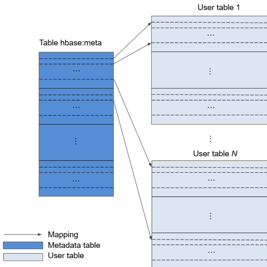
Figure 6-30 Mapping relationships between metadata tables and user tables
