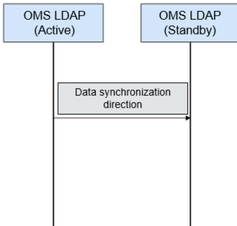
Figure 6-73 OMS LDAP data synchronization
