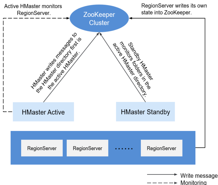
Figure 6-144 Relationship between ZooKeeper and HBase
