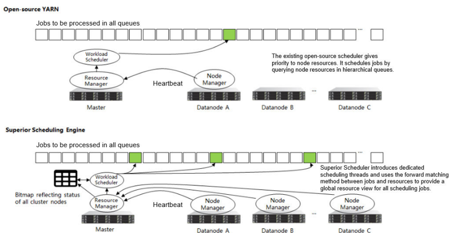
Figure 6-137 Comparison of Superior Scheduler with open source schedulers
