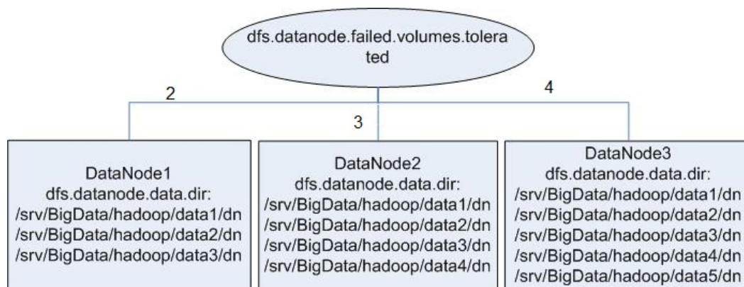
Figure 6-48 Attribute configuration before being enhanced
