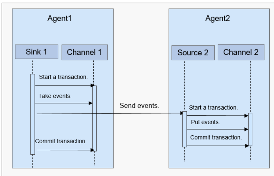
Figure 6-26 Data transmission process
