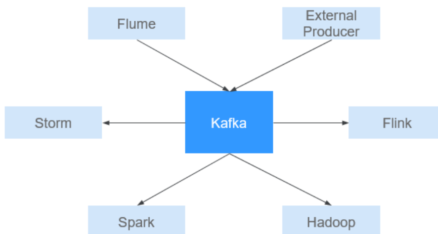
Figure 6-69 Relationships with other components
