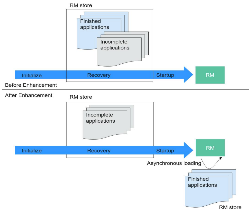
Figure 6-140 Starting the ResourceManager recovery
