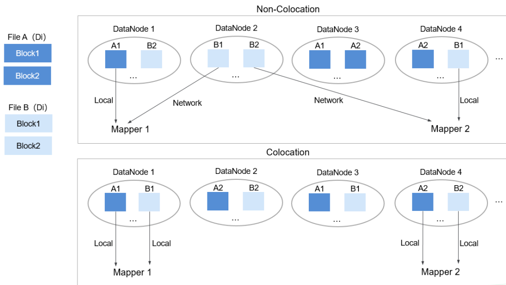
Figure 6-45 Data block distribution in colocation and non-colocation scenarios
