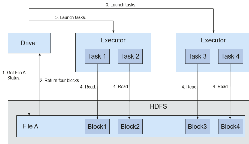
Figure 6-119 File reading process
