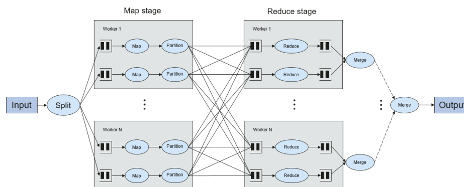
Figure 6-98 Algorithm process
