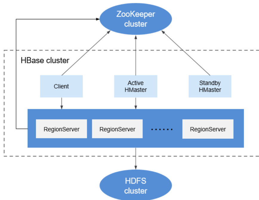
Figure 6-27 HBase architecture
