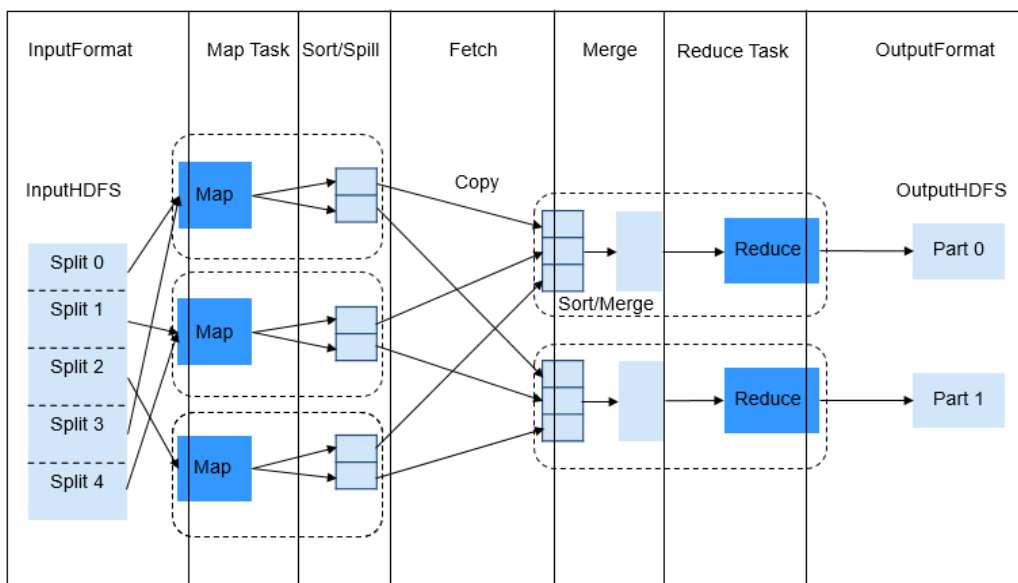
Figure 6-80 MapReduce job
