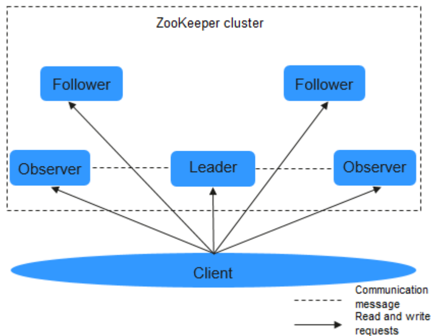
Figure 6-141 Architecture
