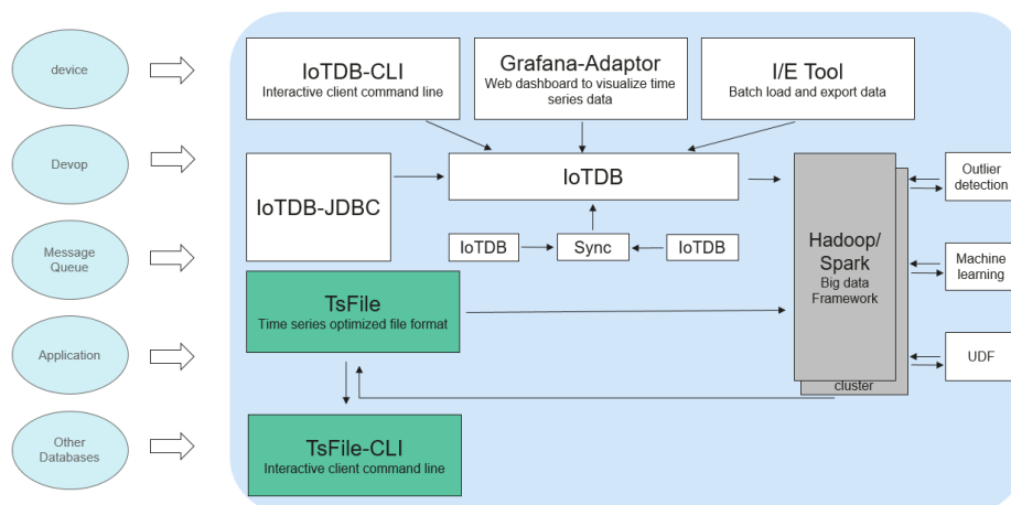
Figure 6-64 IoTDB architecture
