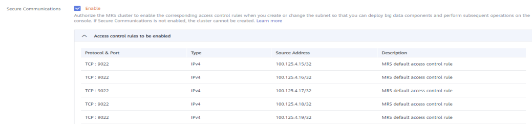
Figure 8-2 Secure communications
