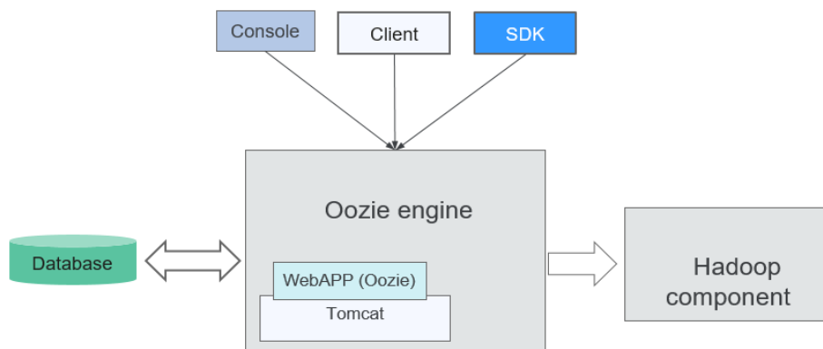
Figure 6-82 Oozie architecture
