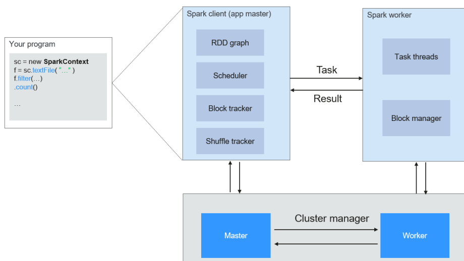
Figure 6-106 Spark application running architecture
