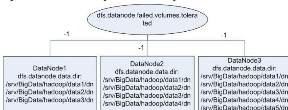
Figure 6-49 Attribute configuration after being enhanced
