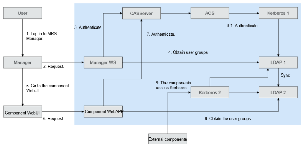
Figure 6-70 Security authentication architecture
