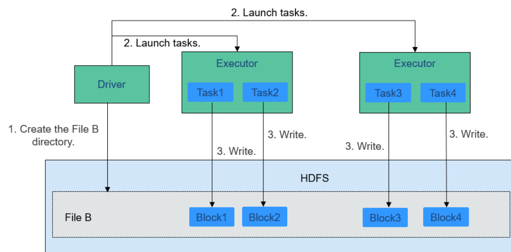
Figure 6-42 File writing process
