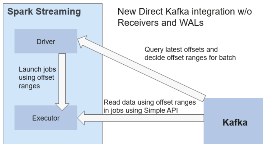
Figure 6-108 Data transmission through Direct Kafka API
