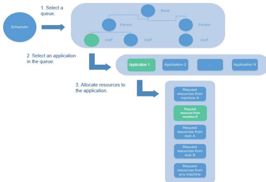
Figure 6-131 Resource allocation model
