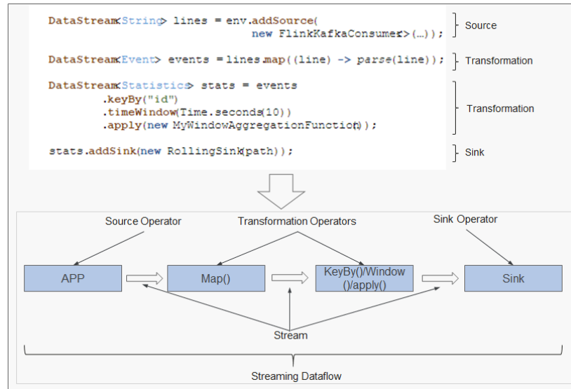
Figure 6-10 Example of Flink DataStream
