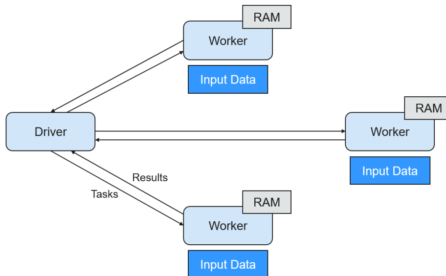
Figure 6-89 Spark Master-Worker mode
