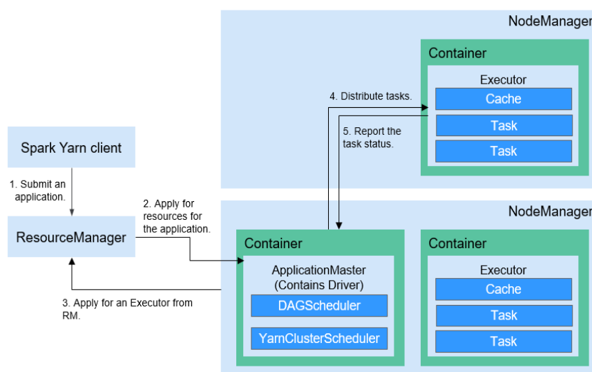
Figure 6-133 Spark on YARN-cluster operation framework
