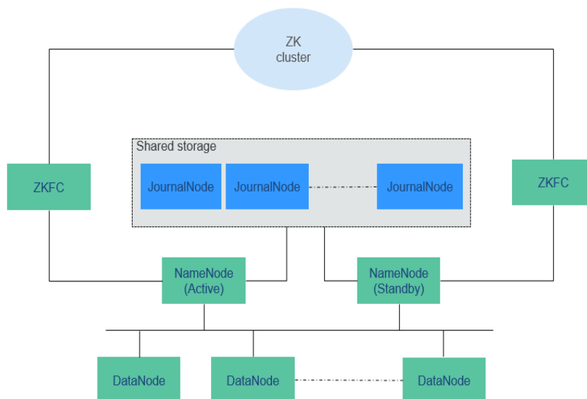
Figure 6-37 HA HDFS architecture
