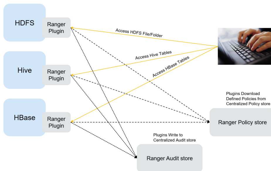
Figure 6-86 Relationships between Ranger and other components
