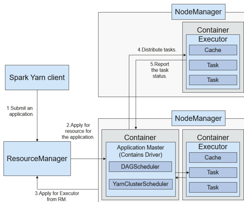
Figure 6-103 Spark on Yarn-cluster operation framework
